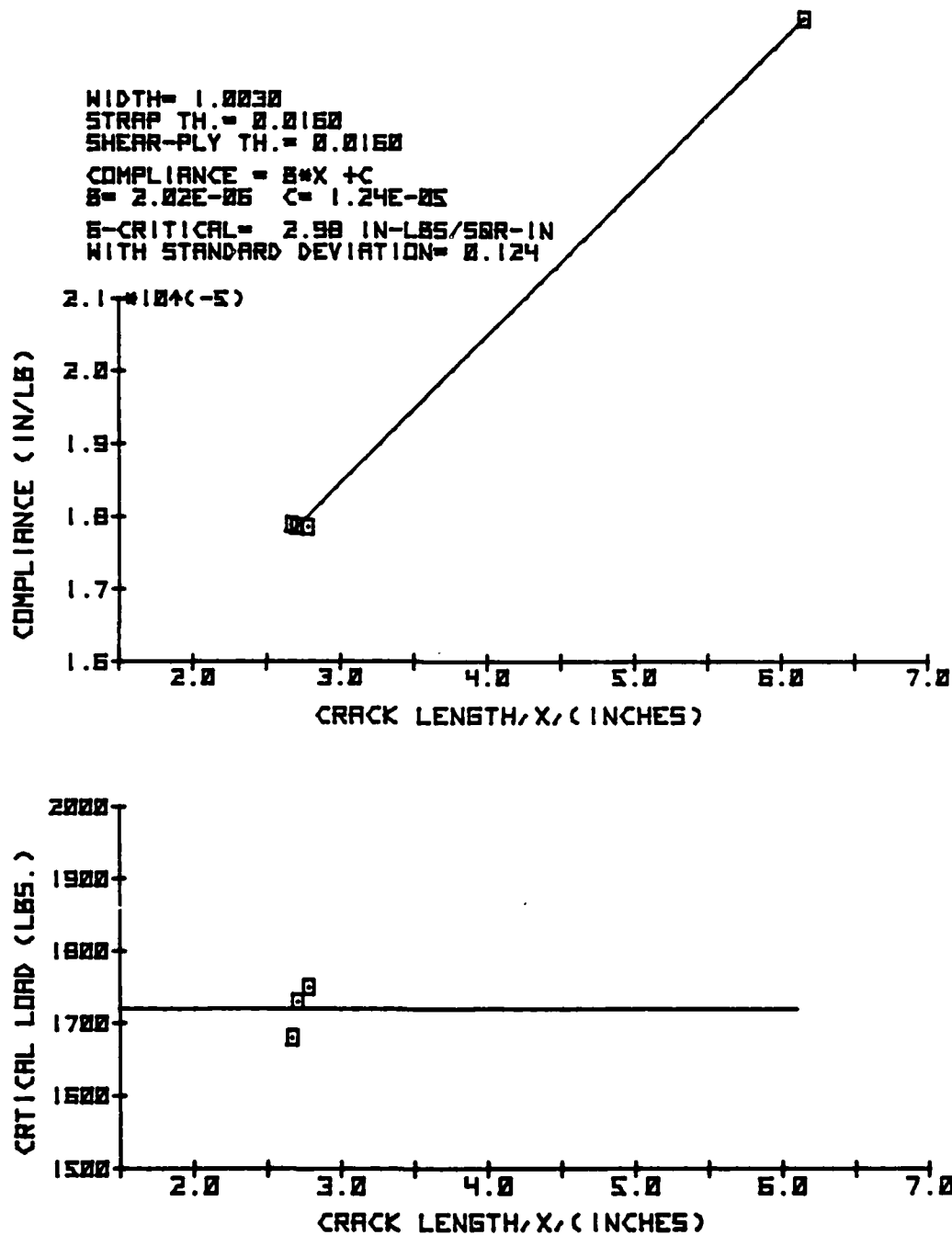
Figure D-10 Test E2CWS of Specimen E2-1-8
