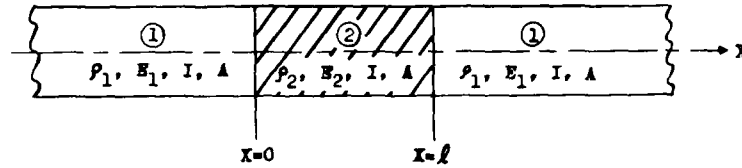
Figure 1.7 - beam of Finite Length Bonded to Two Semi-Infinite Beams Composed of a Different Material
