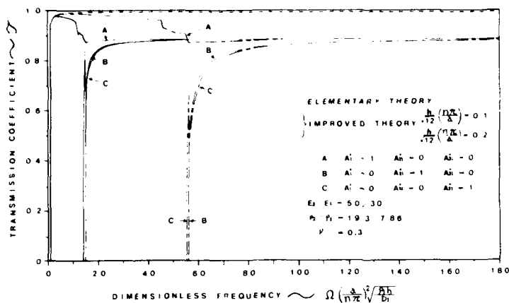
Figure 2.4 - Transmission coefficient vs. frequency, Inhomogeneous Plates
