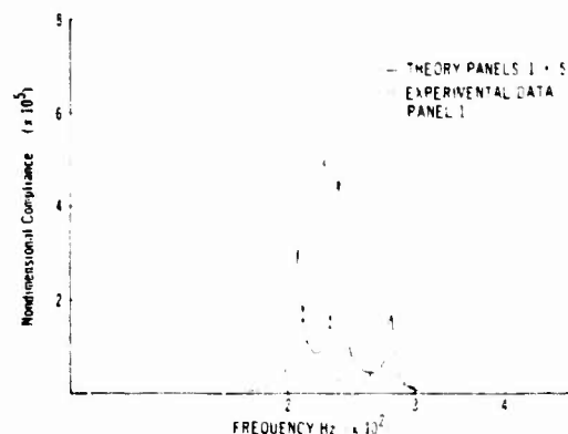
Figure 8. Comparison of Experimentally and Analytically determined Frequency Response of Panel 1 of a Flat Structure.
