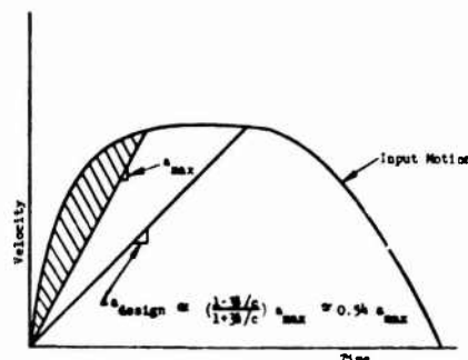
Figure 10. Effect of Translational-Rotational Coupling on Required Rattlespace
