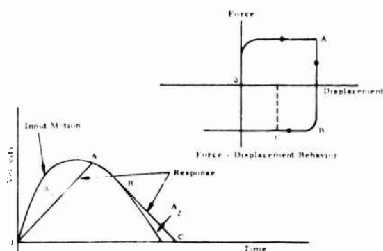
Figure 7. Response Solution for Constant-Force Double-Acting Energy-Dissipative Behavior
