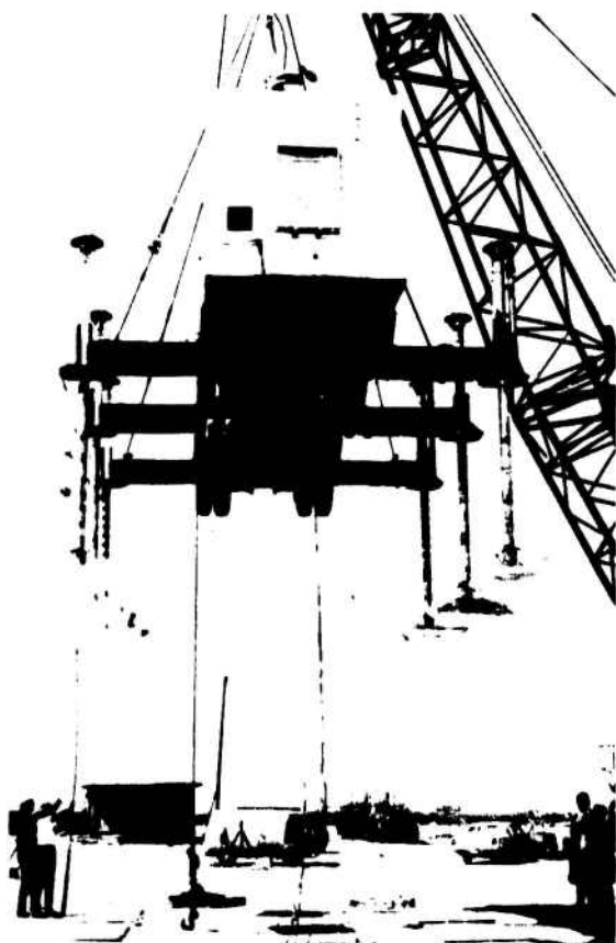
Fig. 6 - Prototype FSGC system ready for 15-ft drop test
