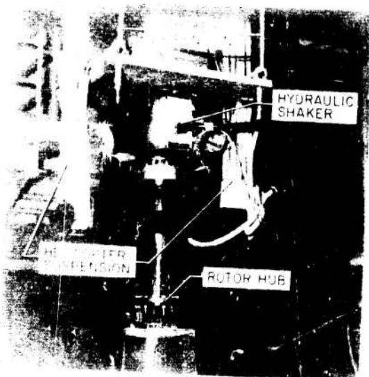
Figure 12. Shaker suspension apparatus.
