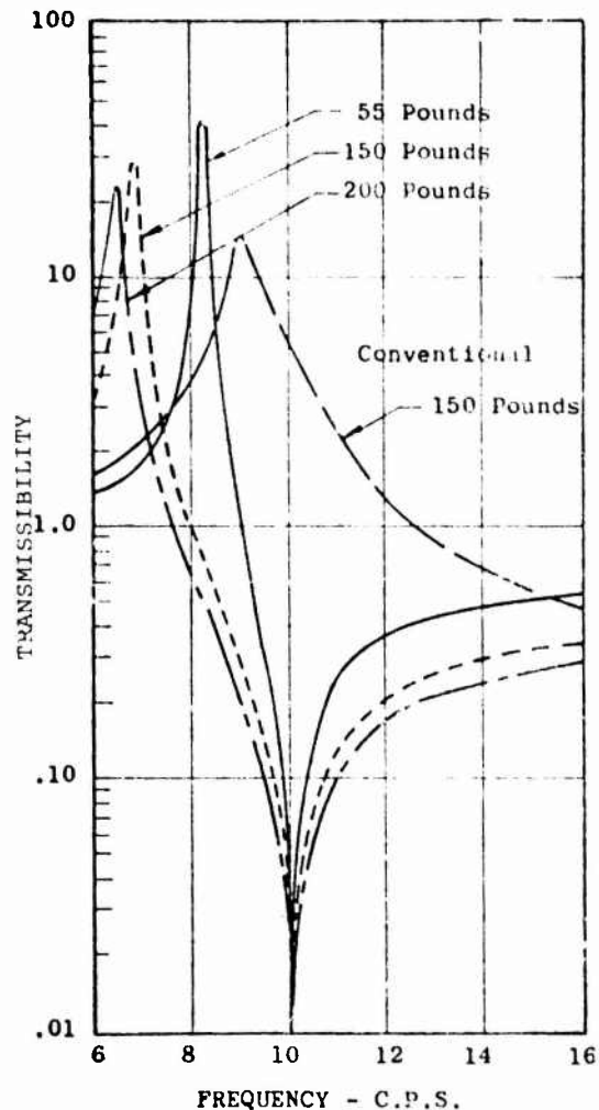
Figure 2. Typical DAVI Transmissibility Curve
