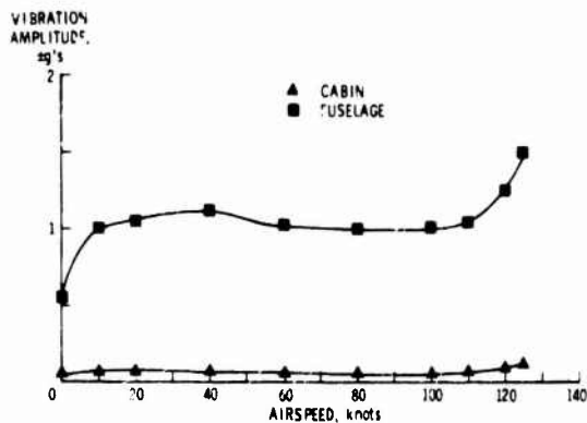
Figure 3. XH-51N 18 Hz vertical vibrations in flight with spring mounted cabin. (Measurement points approximately above and below spring.)
