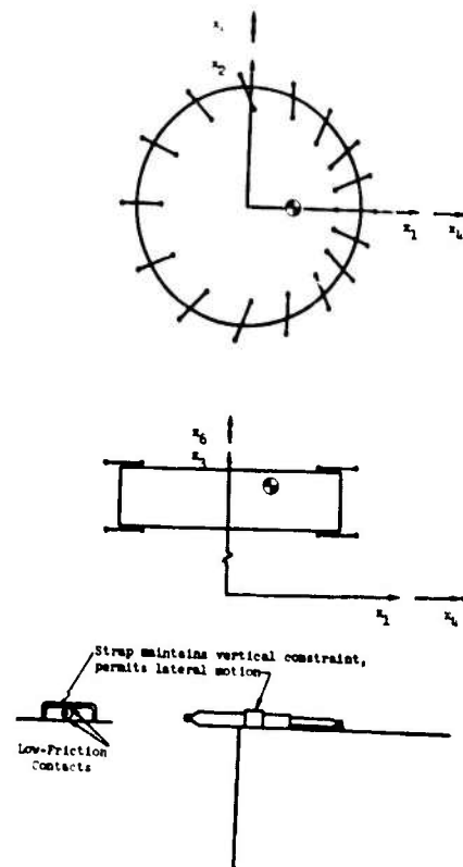
Figure 18. Case I Horizontal Isolation System Used in Parameter Study
