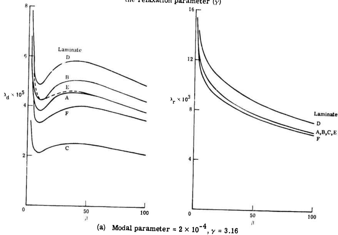
Fig. 3. Variation of damping ( \lambda_d ) and oscillation ( \lambda_r ) coefficients with the intermodal ratio ( \beta )
