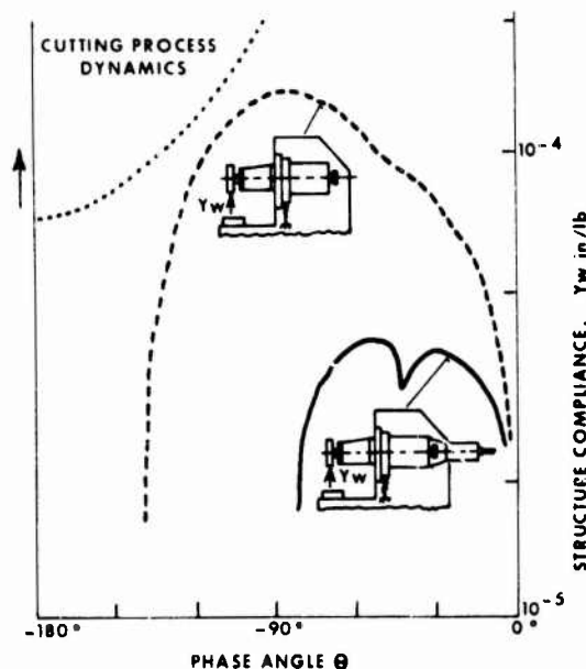
Figure 8 - Gain-Phase Plots as Chatter Onset Indication
