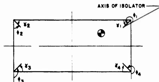
Figure 3: Relationship between \gamma and \psi .
