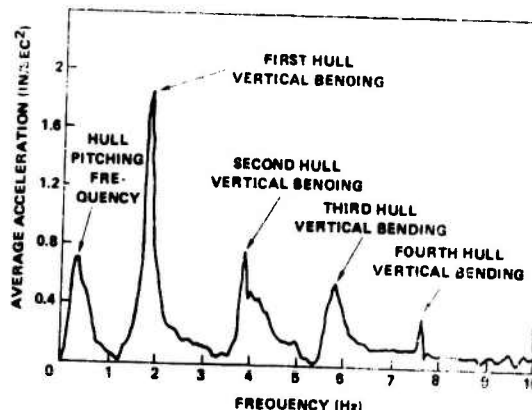
Figure 10 - Hull Stern Vertical Response Spectrum, Run 11
