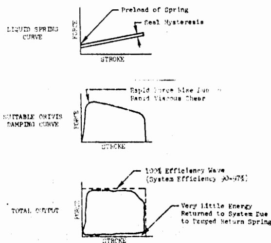
Figure 12. Force-Stroke Curve for a Liquid Spring-Shock with Type 3 Orivis Head Arresting an Impacting Object [6]
