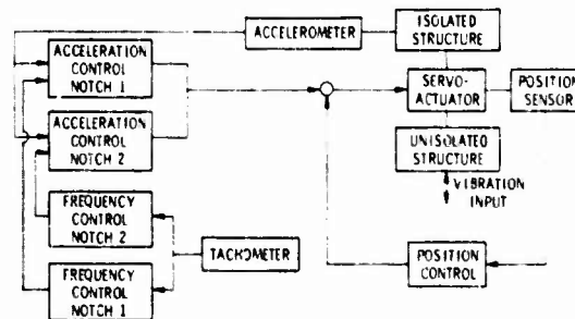
Figure 7. Block diagram of active isolator system.
