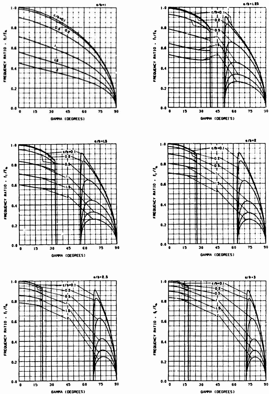
Figure 6: Frequency Ratio, f_1/f_0 versus \gamma
