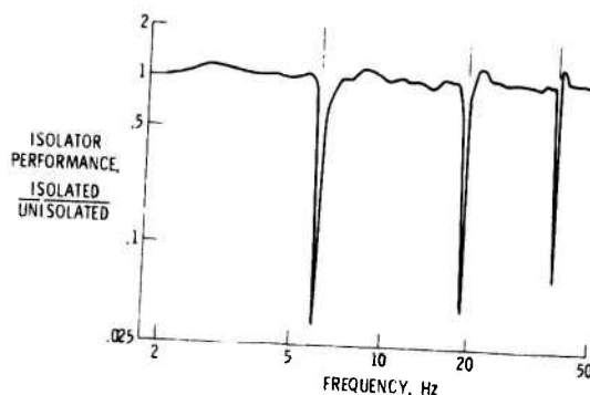
Figure 15. Cabin isolator performance in discrete-frequency tests.
