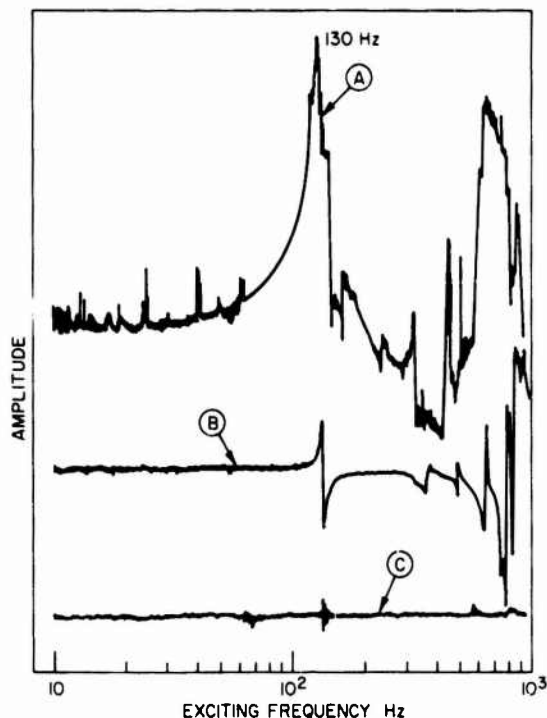
Fig. 3 - Case 3: Rigid body motion of the constraints as a whole. (A) Monitored response signal from the tip of the beam. (B) Monitored response signal from the shake table. (C) Controlled shake table response level.
