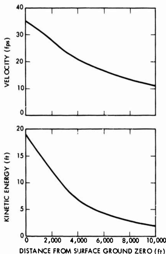
Fig. 1 - Estimated peak vertical surface ground velocity and kinetic energy for Cannikin Event
