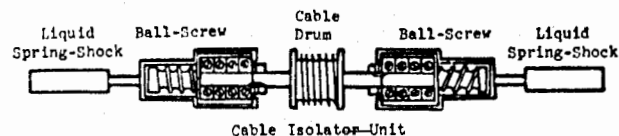
Figure 15. Case I Vertical Isolation System and Cable Isolator Unit
