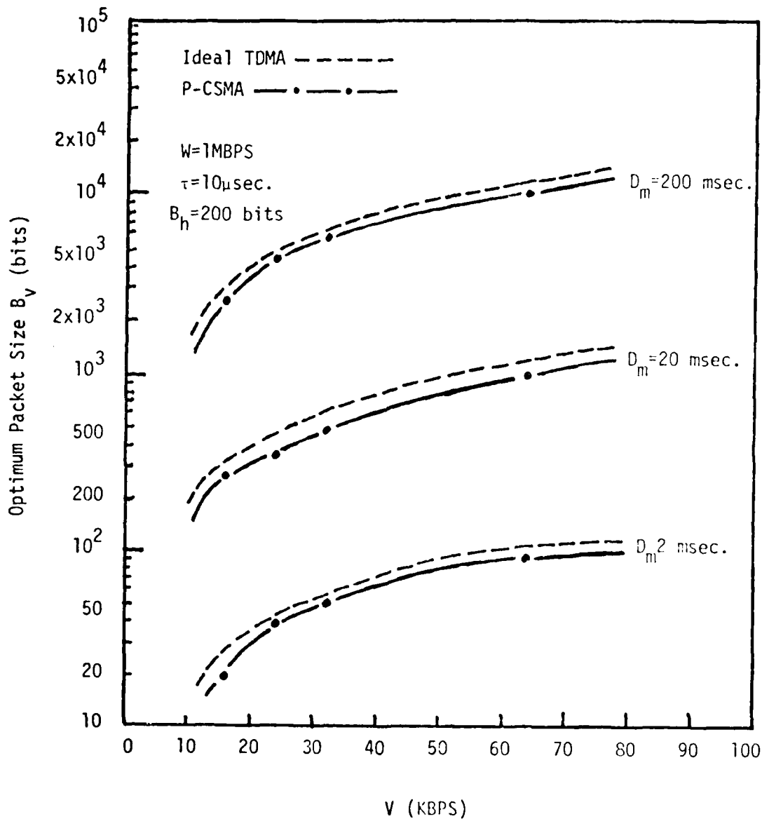
Figure 47. Optimum B_v versus V for W=1\text{MBPS}
