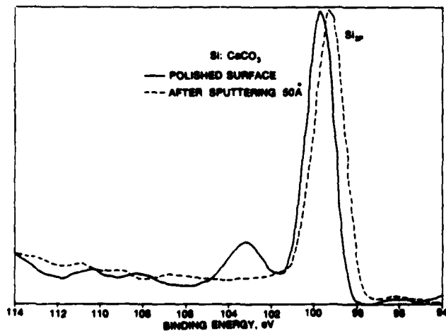
Figure 7. ESCA spectra of a silicon crystal polished with CaCO_3
