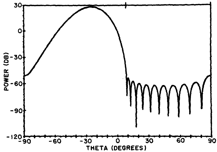
Figure 4b. Eleven Element Pattern: Minimized Sidelobe Sector = [8.46^\circ, 90^\circ]
