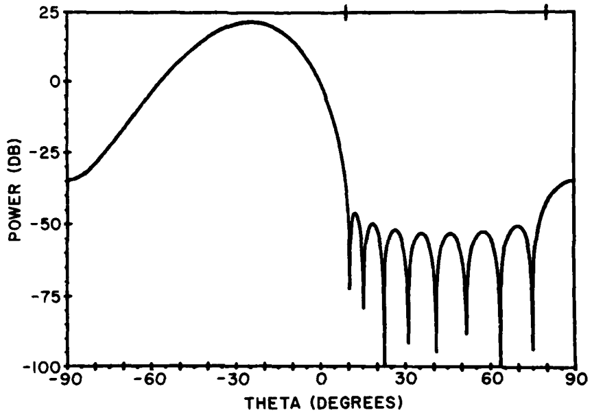
Figure 3a. Nine Element Pattern: Minimized Sidelobe Sector = [9.34^\circ, 80^\circ]
