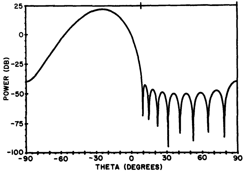
Figure 3b. Nine Element Pattern: Minimized Sidelobe Sector = [8.46^\circ, 90^\circ]
