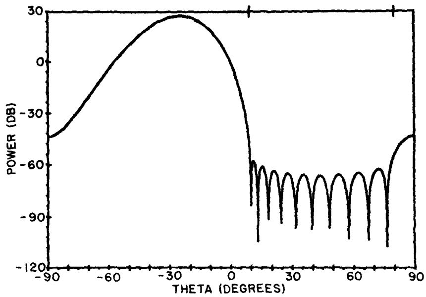
Figure 4a. Eleven Element Pattern: Minimized Sidelobe Sector = [9.34^\circ, 80^\circ]
