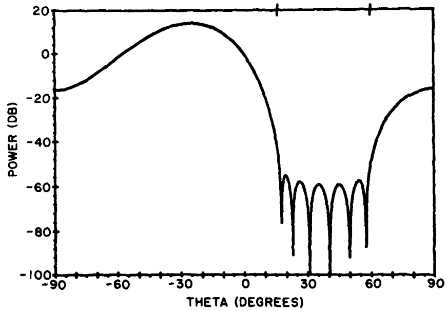
Figure 2b. Seven Element Pattern: Minimized Sidelobe Sector = [16.33°, 60°]
