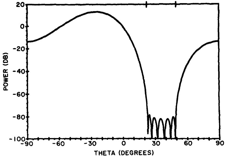
Figure 2a. Seven Element Pattern: Minimized Sidelobe Sector = [22.40°, 50°]
