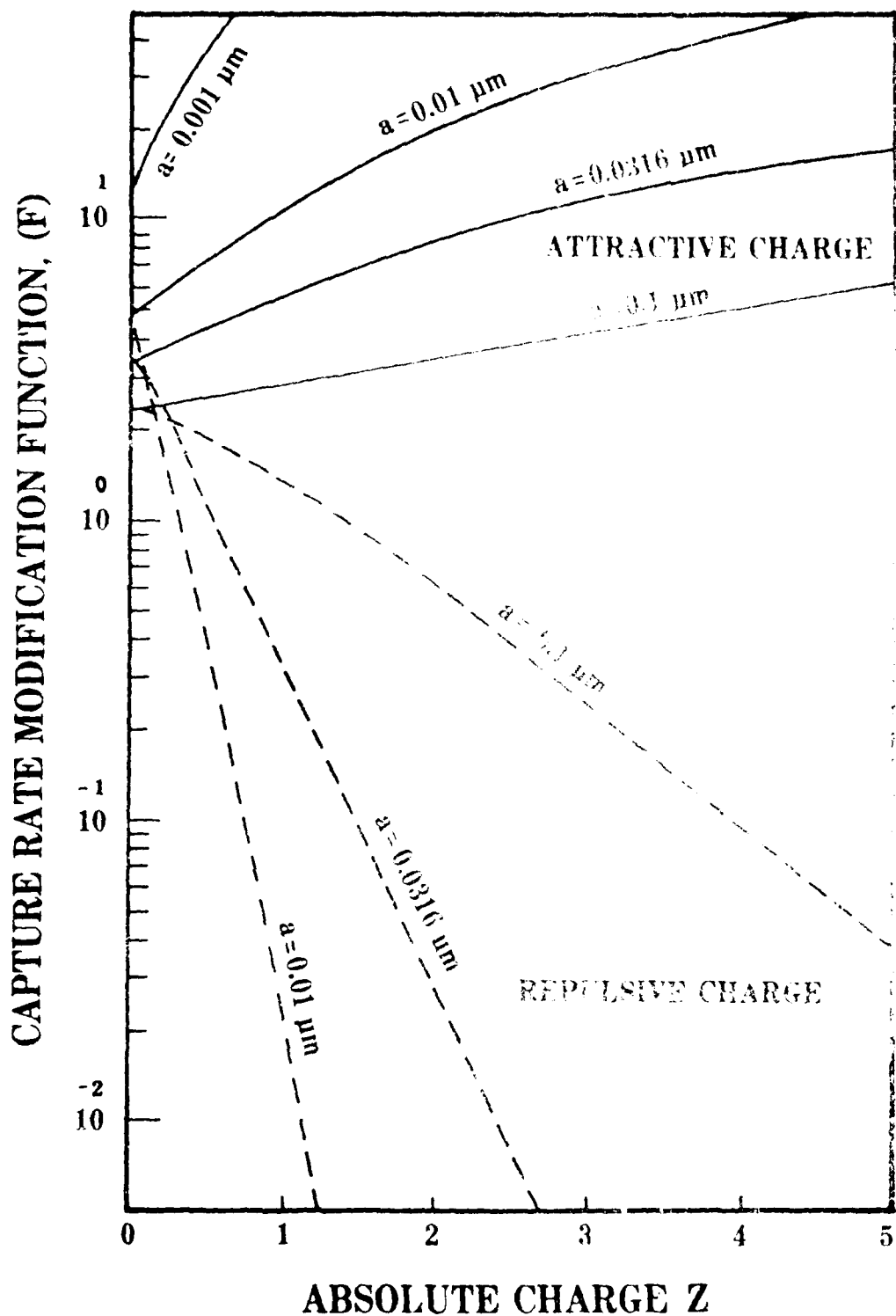
Figure 1. A plot of the capture rate modification function ( F ) against the absolute charge, Z , on a dust particle of radius 0.1 \mu\text{m} to 0.001 \mu\text{m} . The value of the capture rate modification function expresses the ratio of the "effective" capture cross section of a dust particle to the simple geometric cross section and is dependent upon electrostatic effects.
