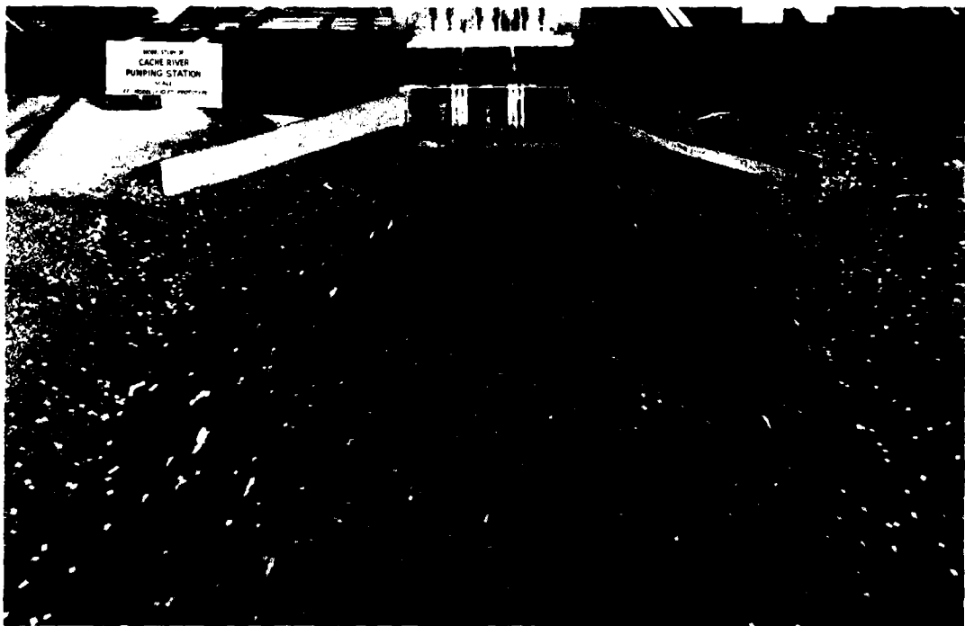
Photo 3. Flow patterns in approach channel, type 1 (original) design; water-surface el 306.0, pumps 1, 2, and 3 operating, 10-sec (prototype) exposure
