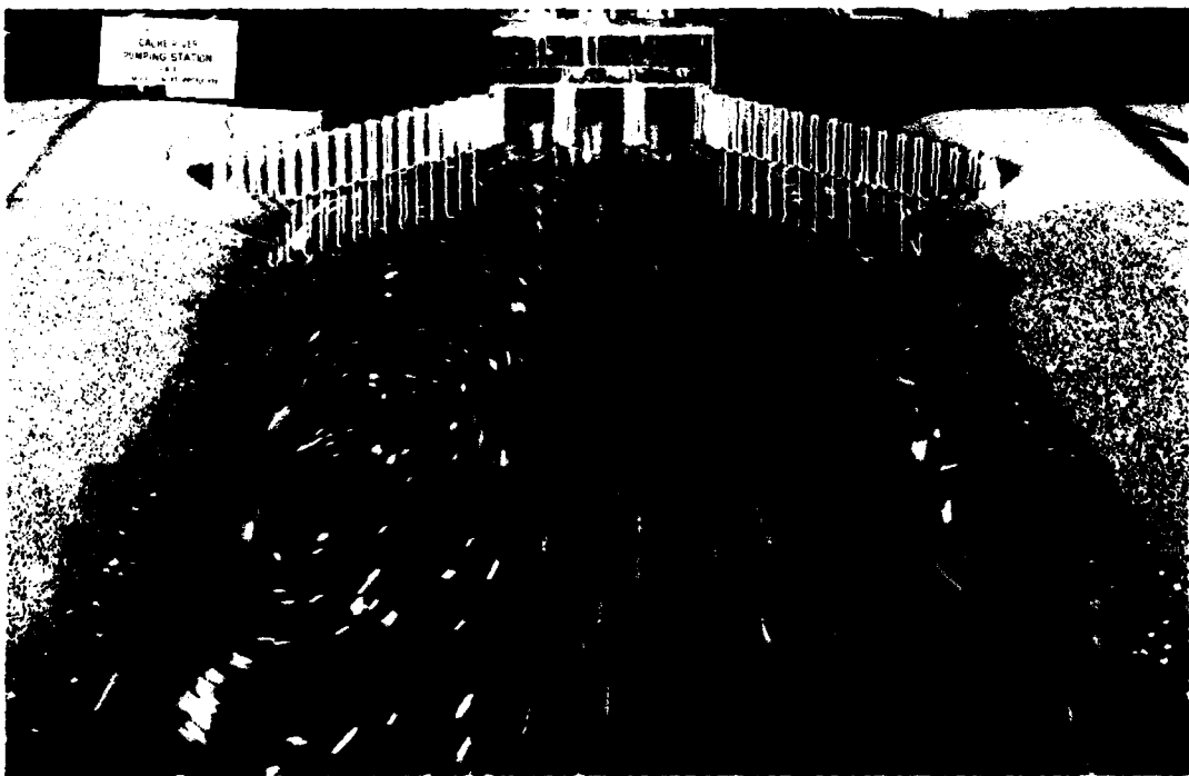
Photo 8. Flow patterns in approach channel, type 2 wing walls; water-surface el 306.0, pumps 2 and 3 operating, 50-sec (prototype) exposure
