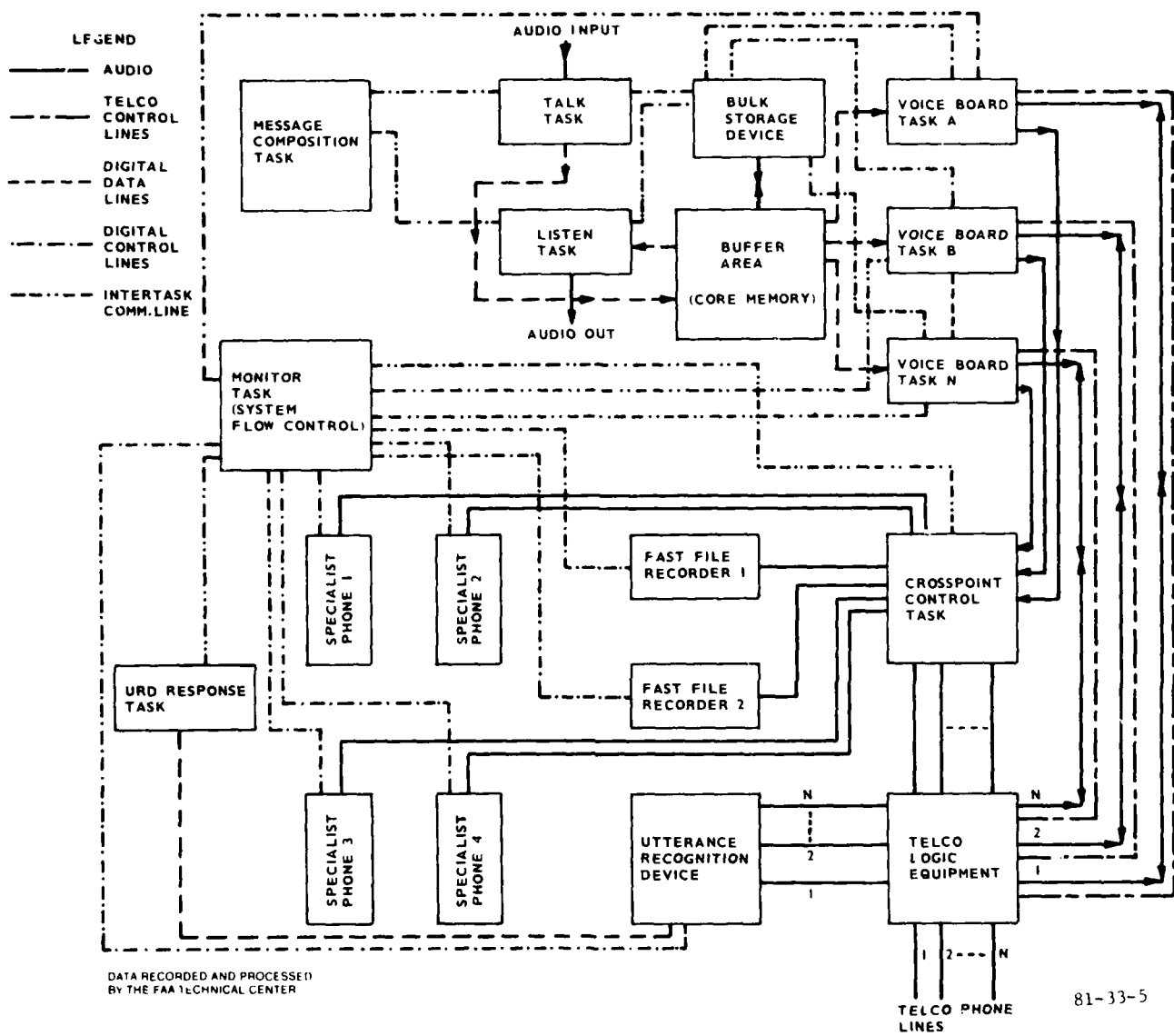
FIGURE 5. FUNCTIONAL BLOCK DIAGRAM OF SYSTEM SOFTWARE
