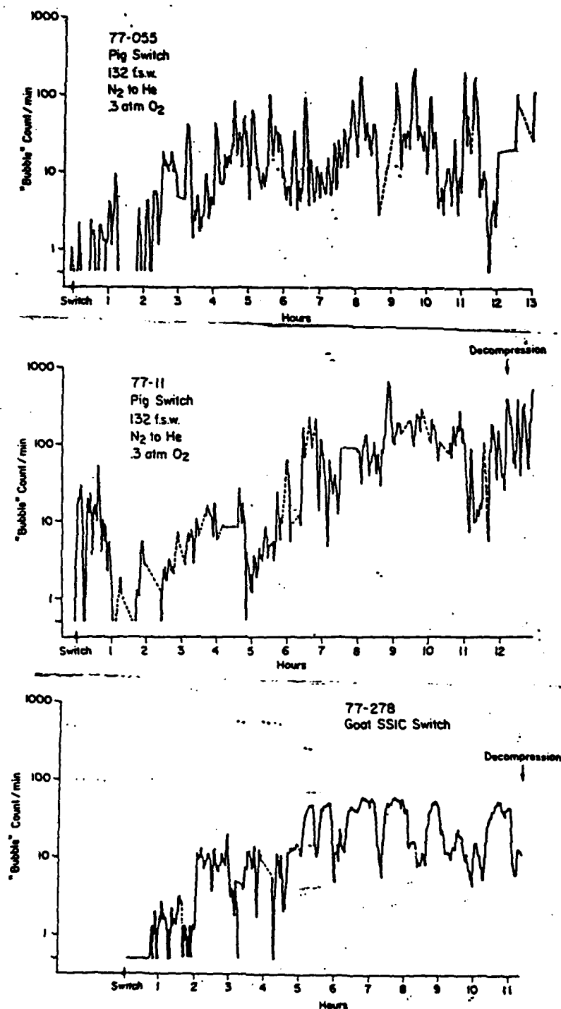
Fig. 20. Comparison of three gas switches, two on a pig with a central venous Doppler bubble detector after a transient gas switch at 132 fsw and one on a goat where only the breathing gas was changed. Note variability in pig experiments, which highly resembles the initial part of the goat experiment. On the other hand, the later part of goat experiment shows much more regular patterns, with an apparent hourly period.
