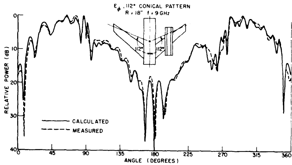
Figure 18. Comparison of measured and calculated near-field patterns for the test geometry. Note that the engine is simulated by flat plates.
