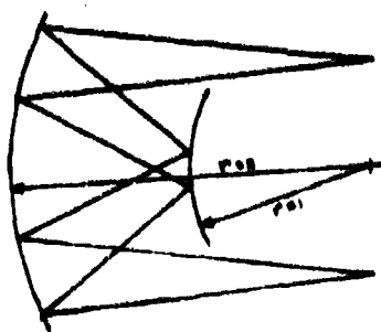
6a. Offner Relay.
