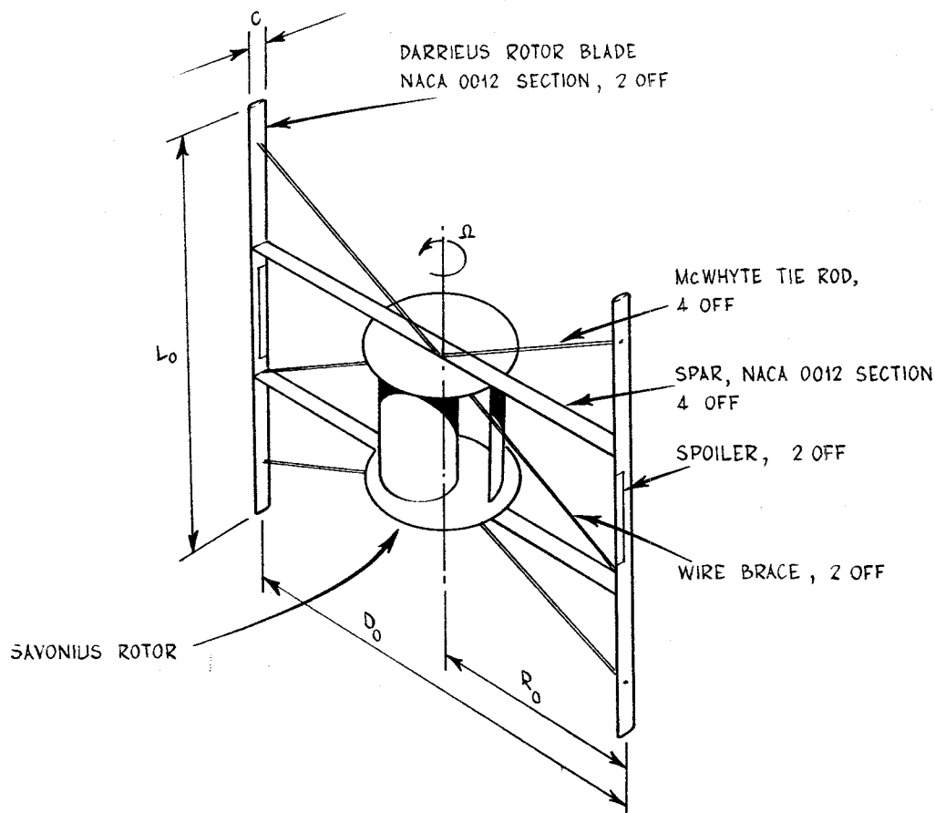
Figure I.1 Turbine scheme
