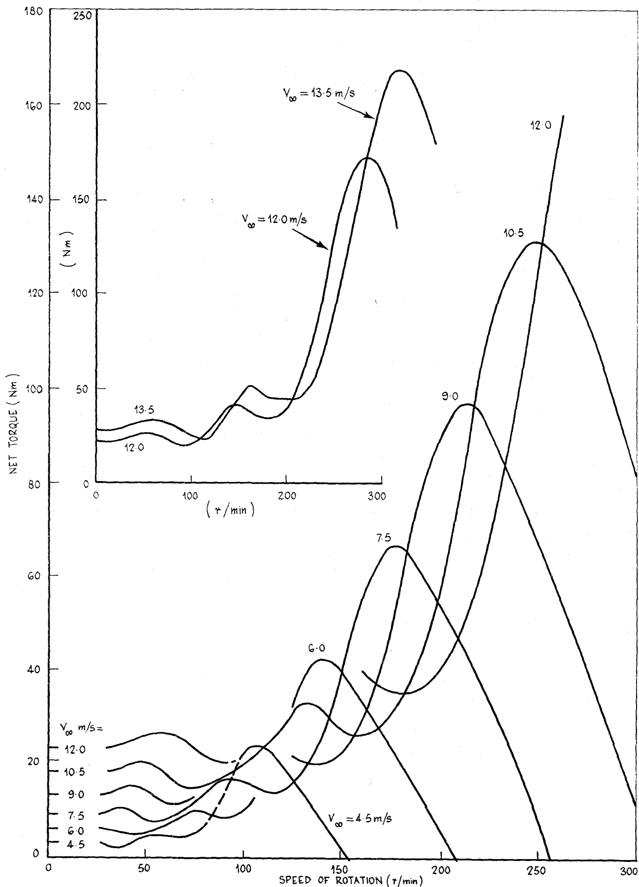
Figure 4. AEL wind-powered generator - variation of net torque of turbine with wind speed and rotational speed
