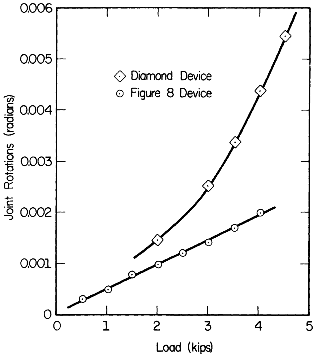
Figure 17. Joint Rotation with Figure Eight and Three inch Diamond Devices.
