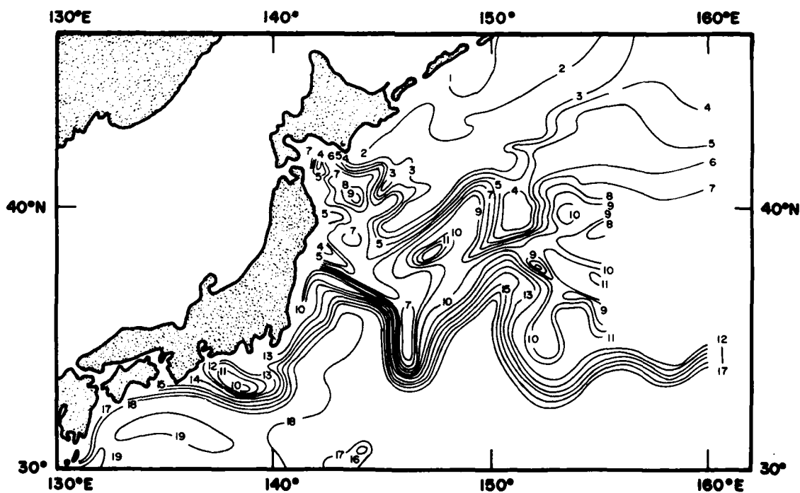
Figure 6.—The 200 meter temperature (°C) distribution for the area of the Kuroshio and the Kuroshio Extension—Winter 1965-66 (after the Provisional CSK ATLAS, 1968).
