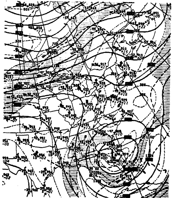
Figure 15. 28/12Z 300-mb Analysis.
