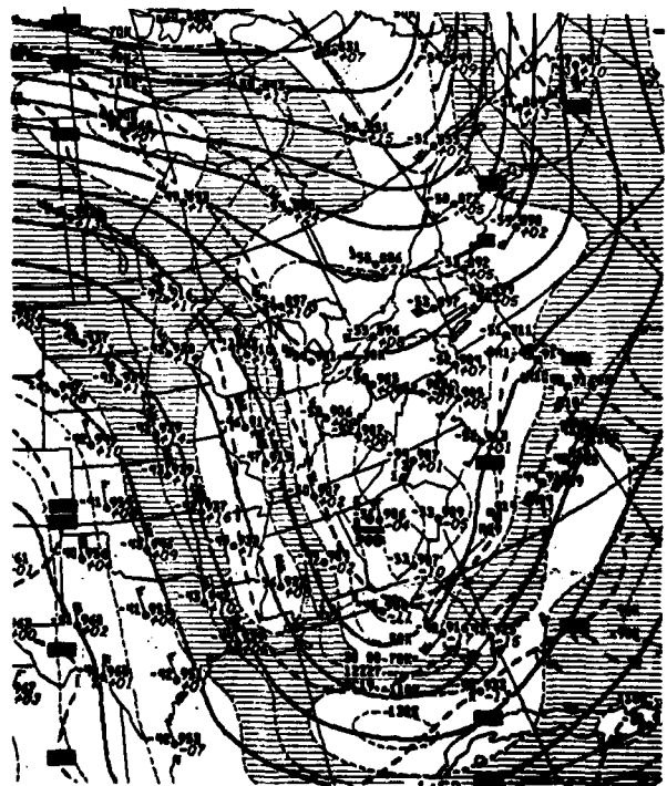
Figure 5. 27/12Z 300-mb Analysis.
