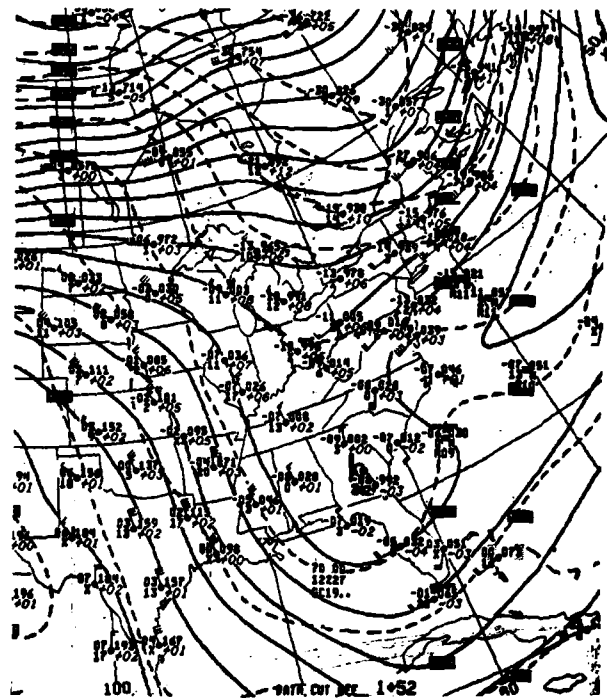
Figure 3. 27/12Z 700-mb Analysis.
