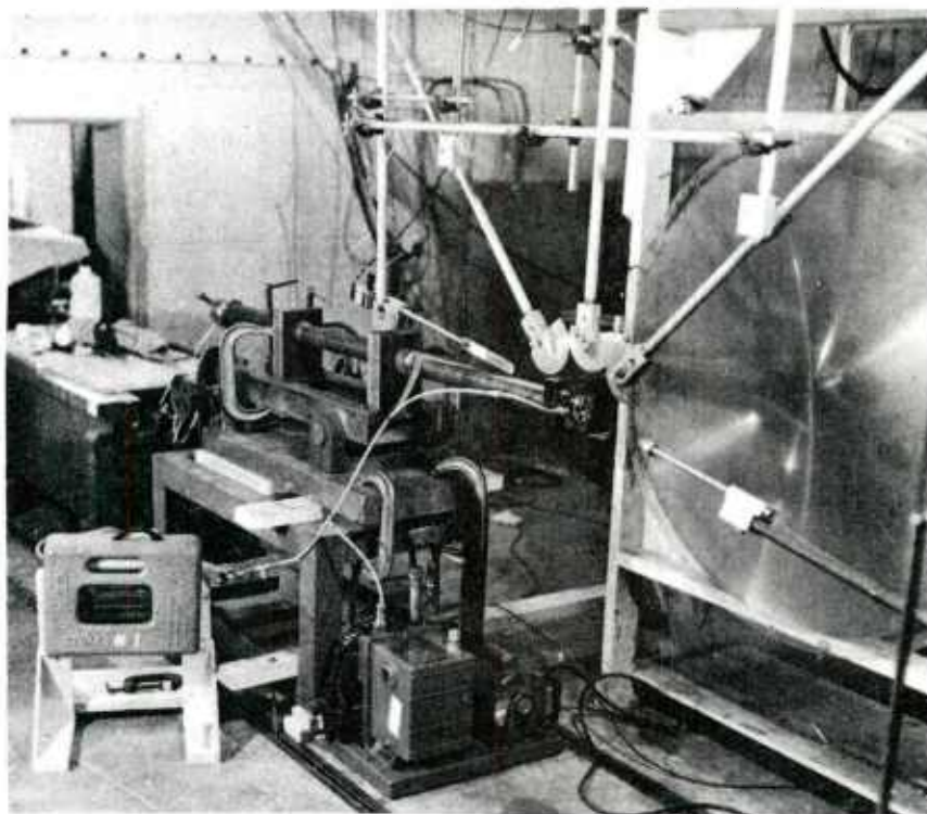
Figure 2. Experimental Instrumentation
