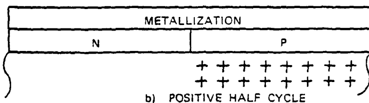
b) POSITIVE HALF CYCLE
