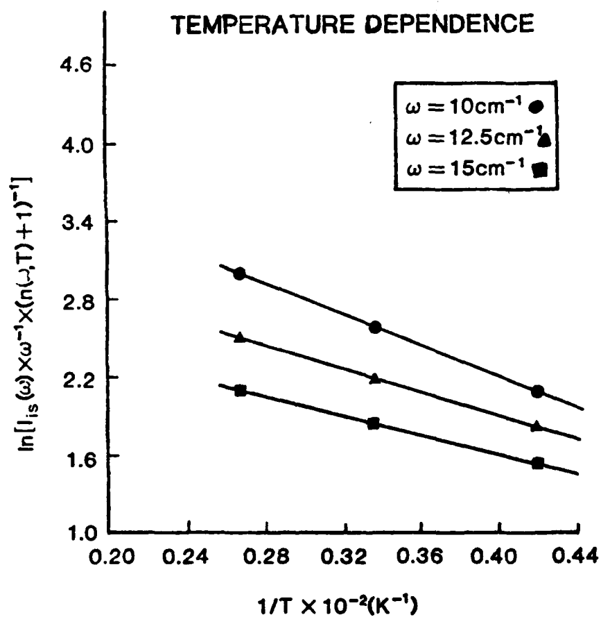
Figure 6(c). Low frequency Raman spectrum of optical fibers showing the natural logarithm of the intensity as a function of reciprocal temperature.
