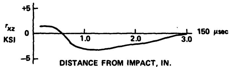
Figure 11. Shear Stress r_{xz} Vs. x Distance From Impact Point For Given Times Shown On Right Hand Side.
