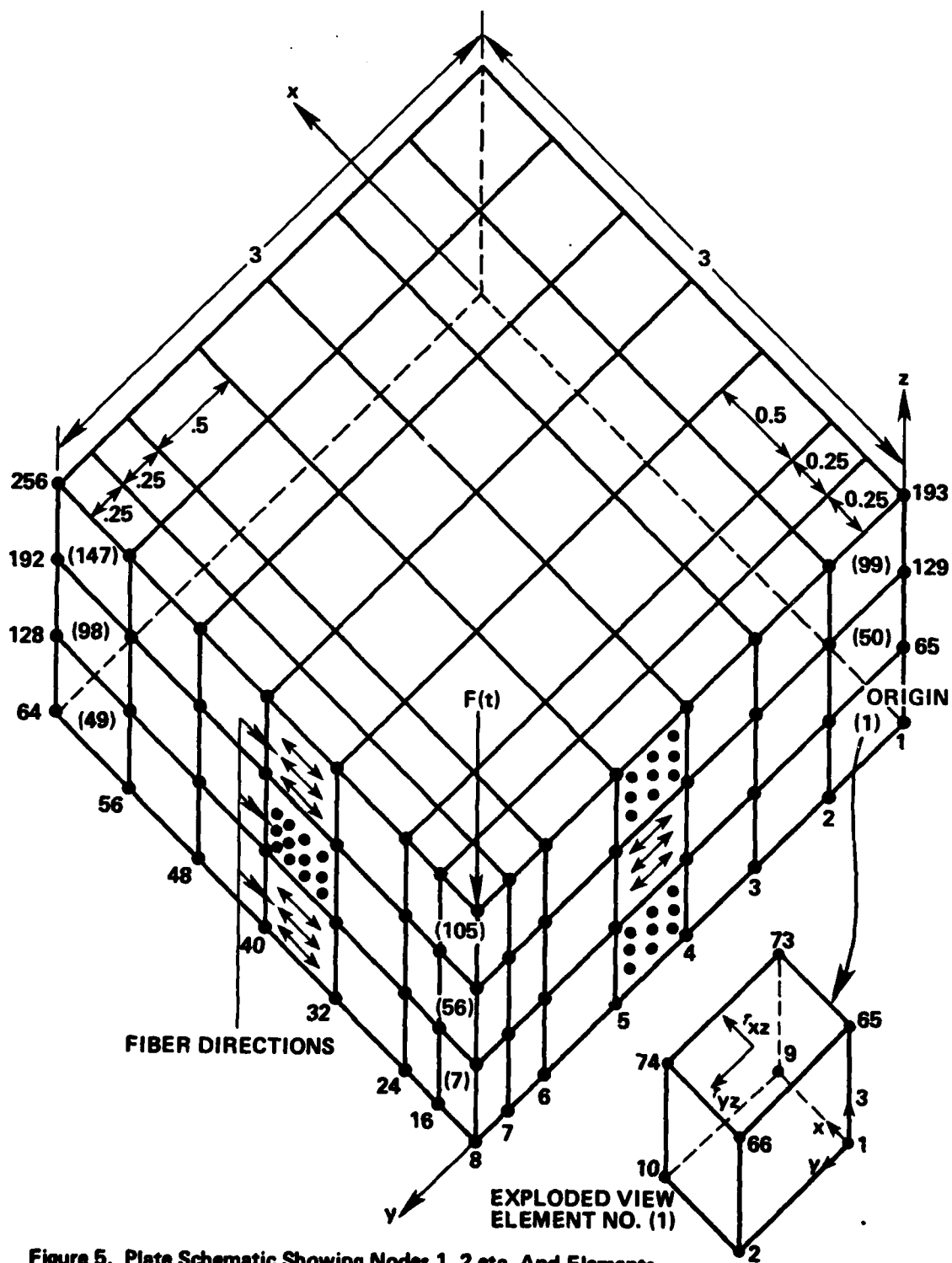
Figure 5. Plate Schematic Showing Nodes 1, 2 etc. And Elements (1), (2) etc. Drawing Not to Scale Node No. 8 is Bottom Center Point. Load is Applied at Node No. 200, Top Center Point.
