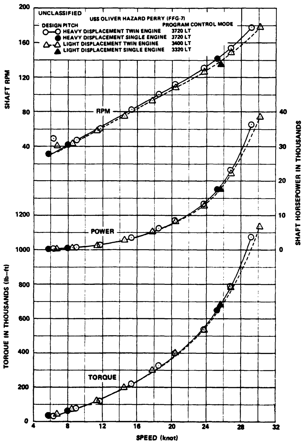
Figure 3 - Comparison of Heavy and Light Displacement Standardization Trial Results, English Units (U)
