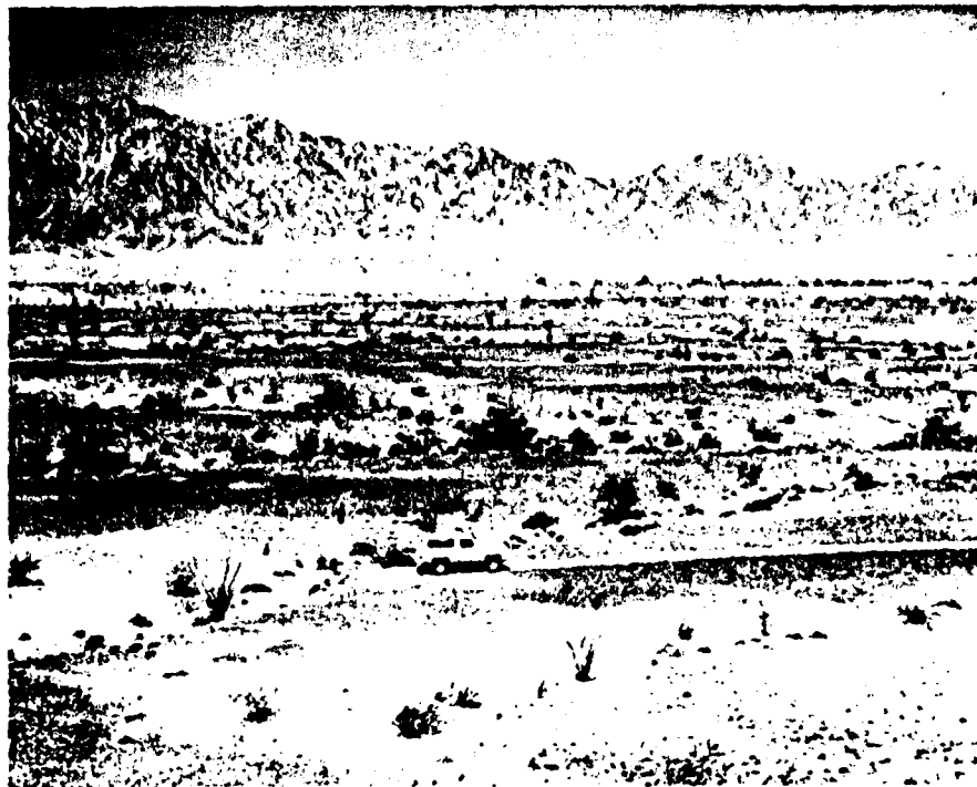
Well developed desert pavement and patina of intermediate alluvial fan surface (A5i; Section 4.4.2.3). Smooth sparsely vegetated surface is undergoing dissection by modern drainages eroding headward near Gila Mountains (background) and flowing to the north. View west across older alluvial fans (A5o; Section 4.4.2.4).
