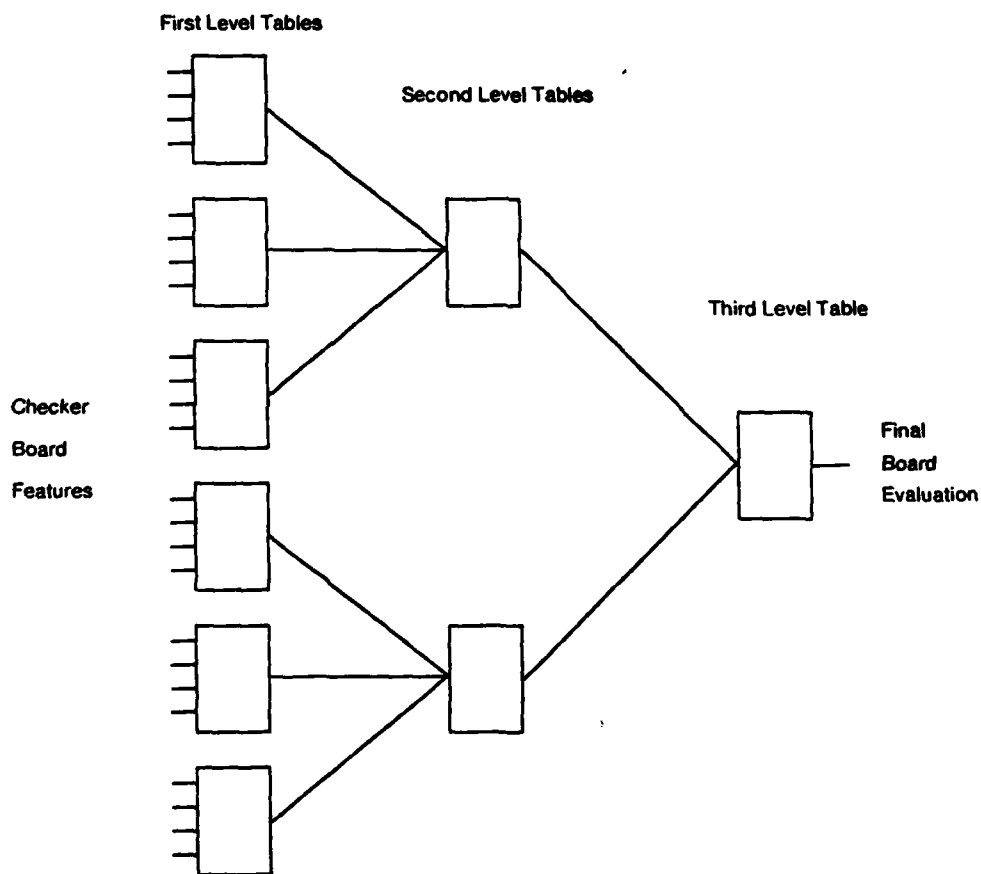
Figure 4-2: Samuel's three-level signature table scheme.
