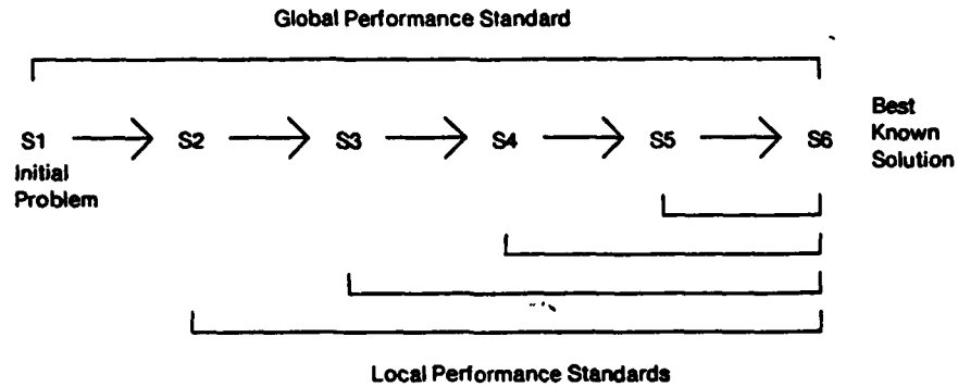
Figure 2-1: Global and local performance standards in LEX.
