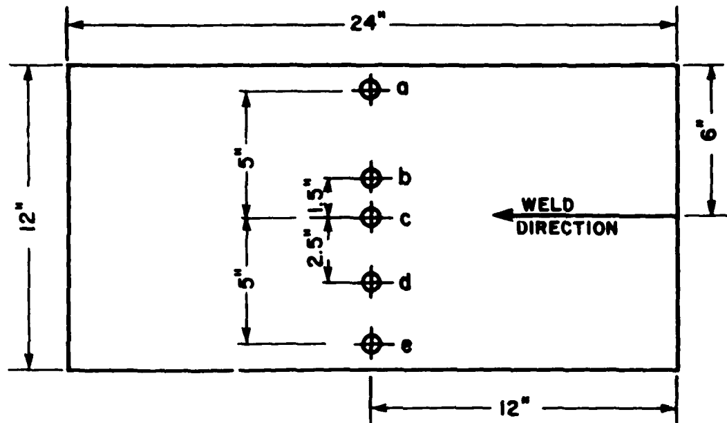
FIGURE 4.5 Dial indicator locations for Specimens #1 through #6
