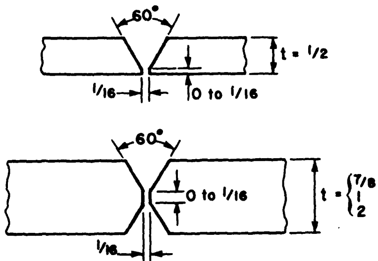
FIGURE 2.1 Configuration of simple restrained specimens. (Dimensions are in inches)
