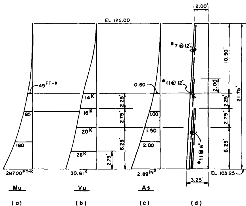
Figure 5. Stem - moments, shears, and reinforcement
