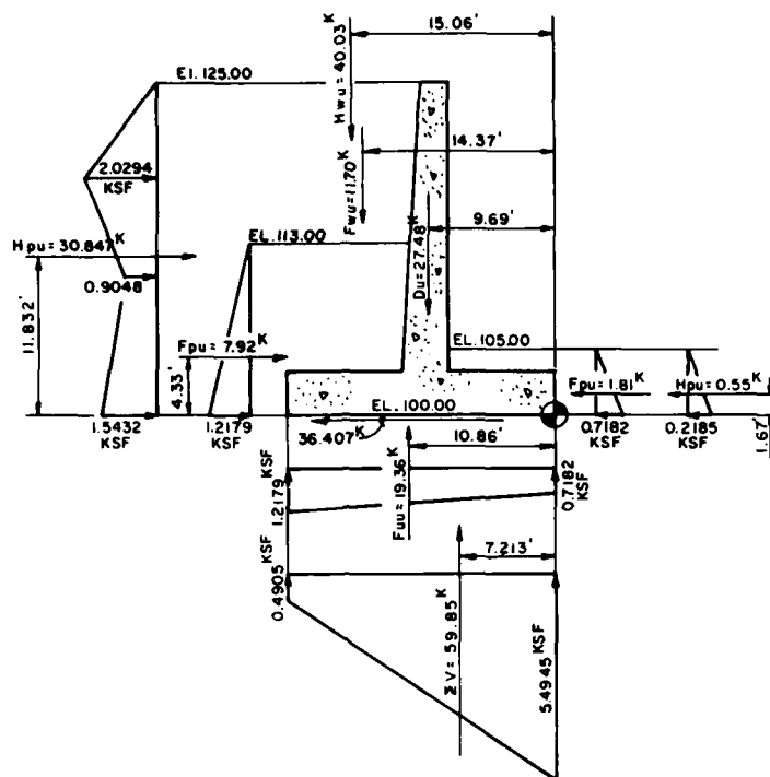
Figure 4. Loading diagram for factored loads
