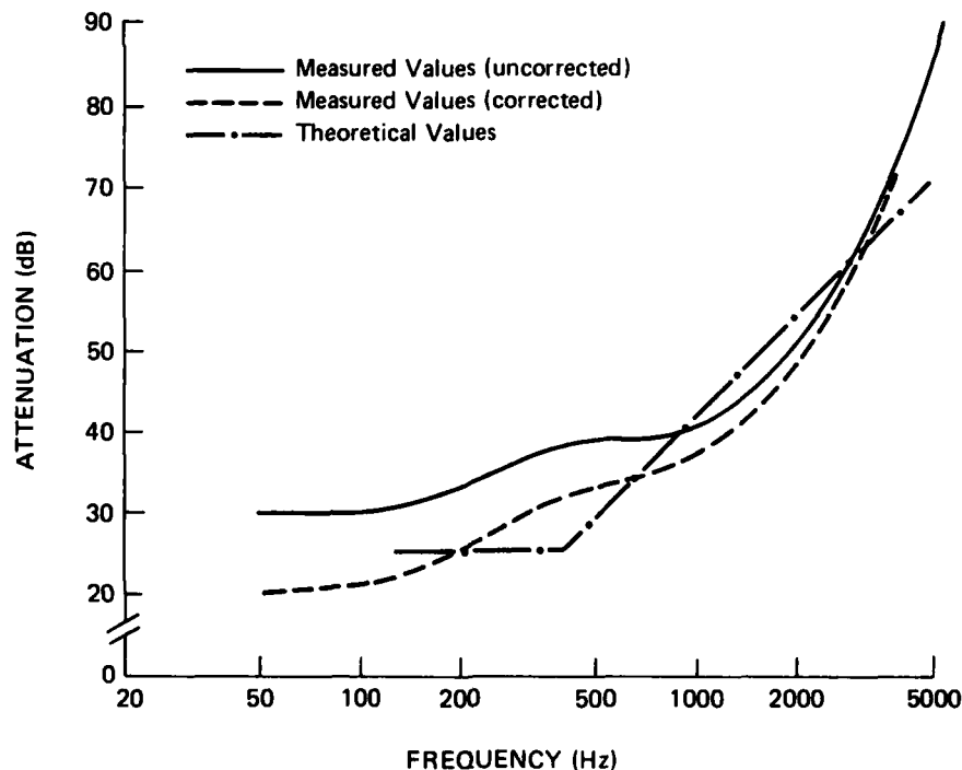
FIGURE A-1 Attenuation of external sound through maternal tissues.
