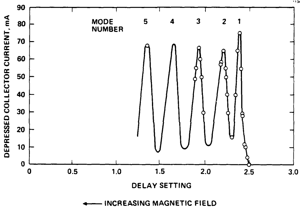
Figure 27. Depressed collector current as a function of delay setting, V_{\text{anode}} = 19 kV.
