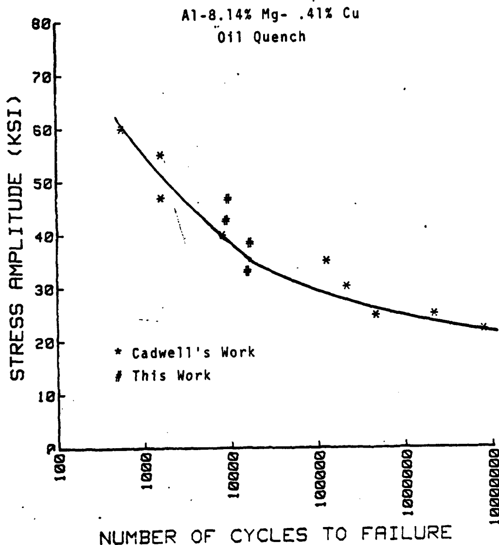
Figure 16. Stress-Amplitude vs Cycles-to-Failure for Al-8.14%Mg-0.41%Cu, solution treated and forged @ 440°C, oil quenched and warm rolled @ 300°C; *Cadwell's work [Ref. 8] - 10-hour solution treatment, #This work - 24-hour solution treatment.
