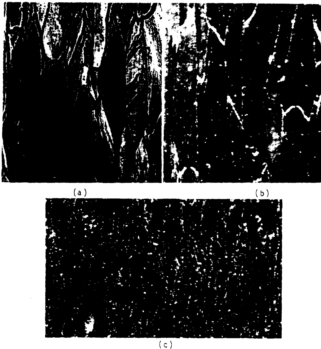
Figure 13. Optical micrographs of Al-10.2%Mg, solution treated @ 440°C, forged, quenched and warm rolled @ 300°C: (a) 10-hour solution treatment, oil quenched, (b) 24-hour solution treatment, oil quenched, (c) 24-hour solution treatment, water quenched. (300X)
