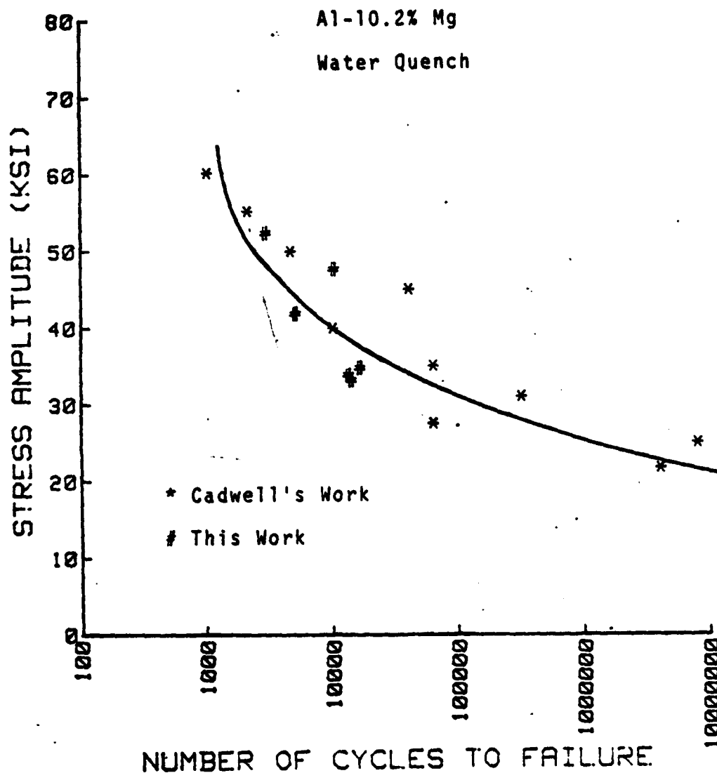
Figure 19. Stress-Amplitude vs Cycles-to-Failure for Al-10.2%Mg, solution treated and forged @ 440°C, water quenched and warm rolled; *Cadwell's work [Ref. 8] - 10-hour solution treatment, #This work - 24-hour solution treatment.
