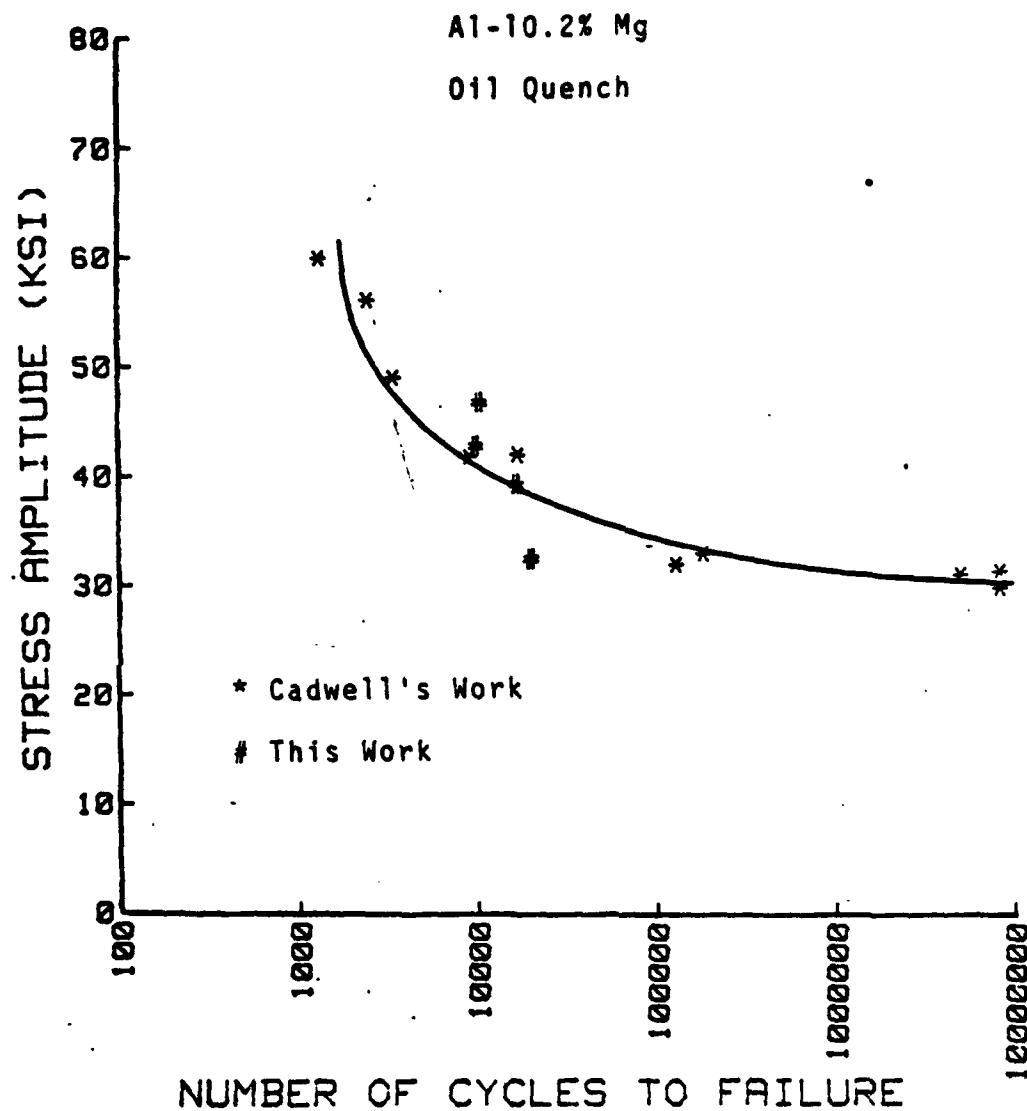
Figure 18. Stress-Amplitude vs Cycles-to-Failure for Al-10.2%Mg, solution treated and forged @ 440°C, oil quenched and warm rolled; *Cadwell's work [Ref. 8] - 10-hour solution treatment, #This work - 24-hour solution treatment.
