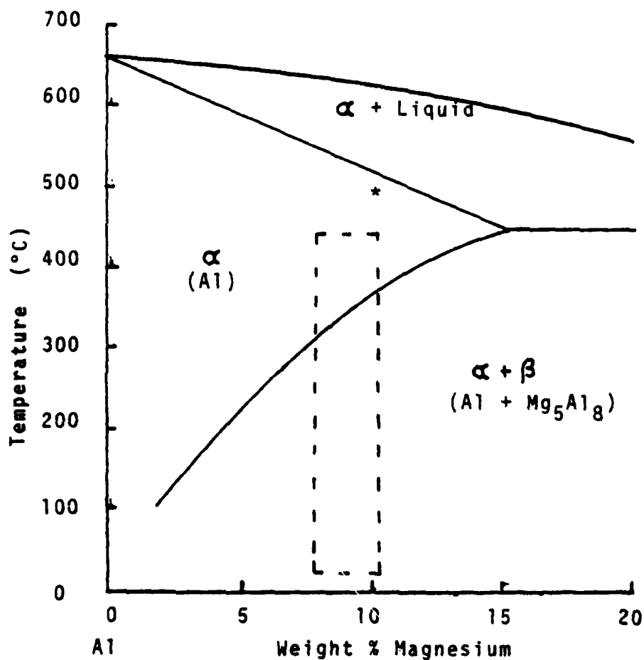
Figure 1. Partial Aluminum-Magnesium Phase Diagram. Dashed in area represents compositions used in this work. * Represents the solution treatment temperature used on the Al-10.2%Mg -0.52%Mn alloy.
