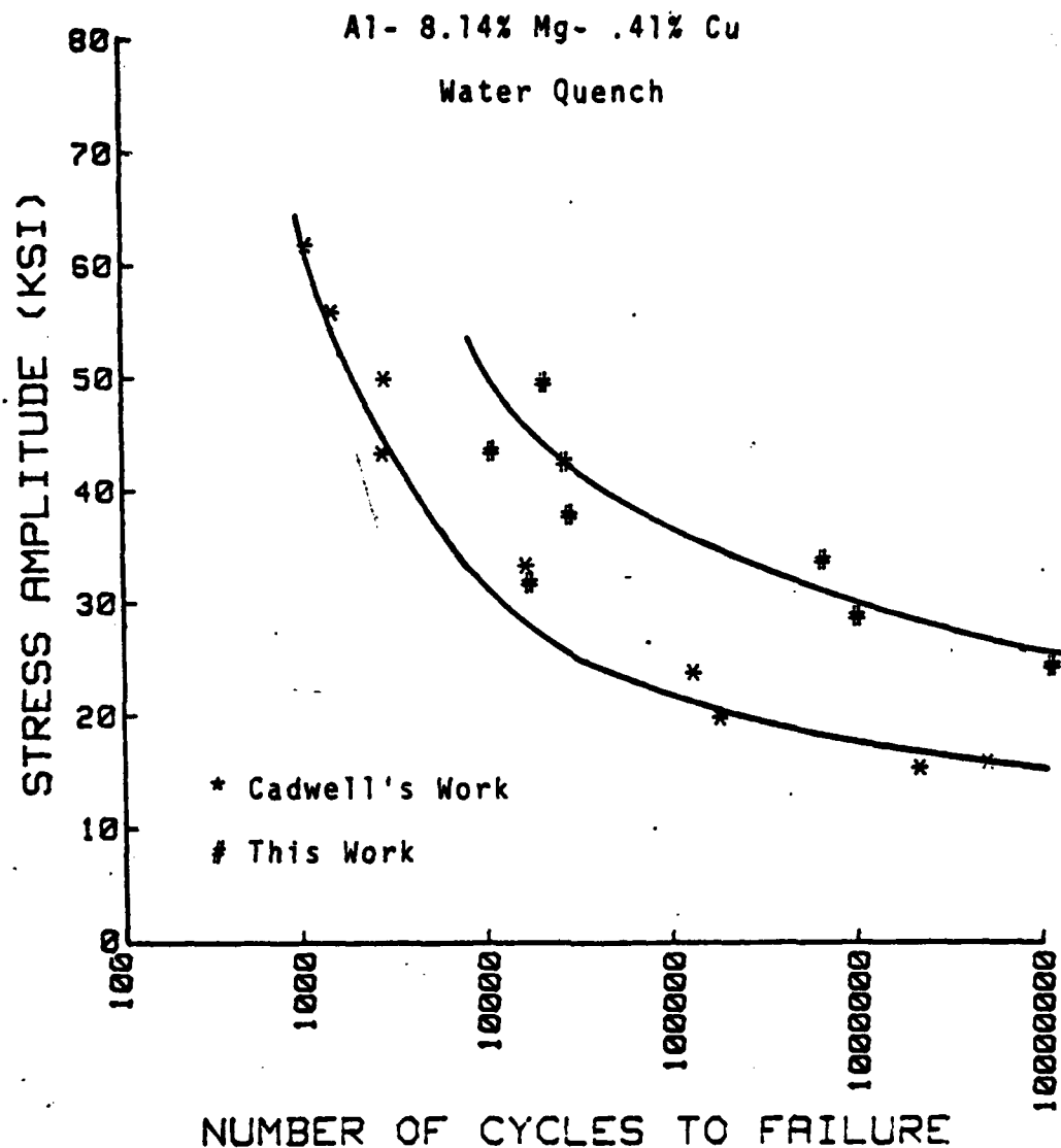
Figure 17. Stress-Amplitude vs Cycles-to-Failure for Al-8.14%Mg-0.41%Cu, solution treated and forged @ 440°C, water quenched and warm rolled @ 300°C; *Cadwell's work [Ref. 8] - 10-hour solution treatment, #This work - 24-hour solution treatment.
