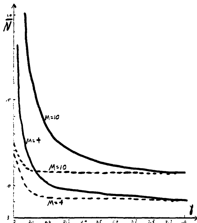
Fig. 1. Average backlog of a user in TDMA system as a function of the rate of traffic variation.
