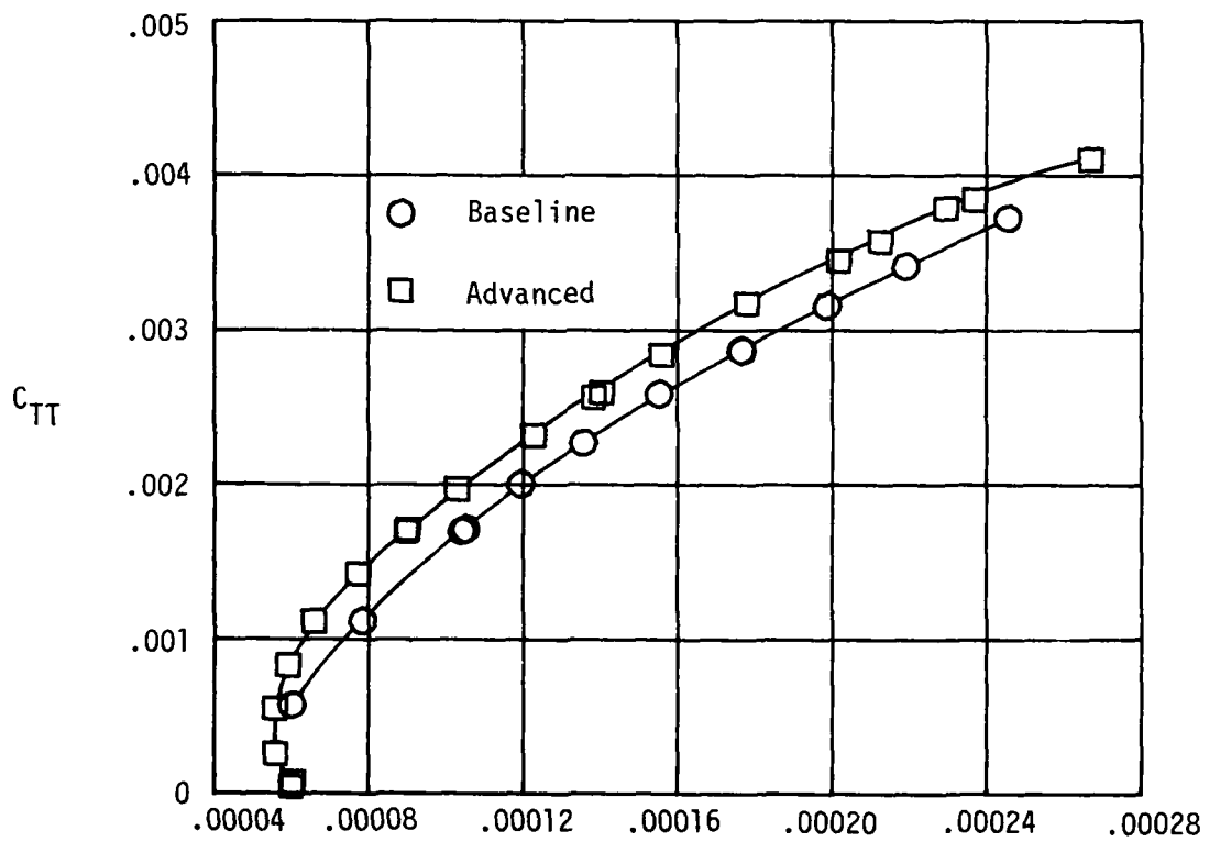
Figure 5.- Comparison of net hover performance of rotor-blade sets out of ground effect.
