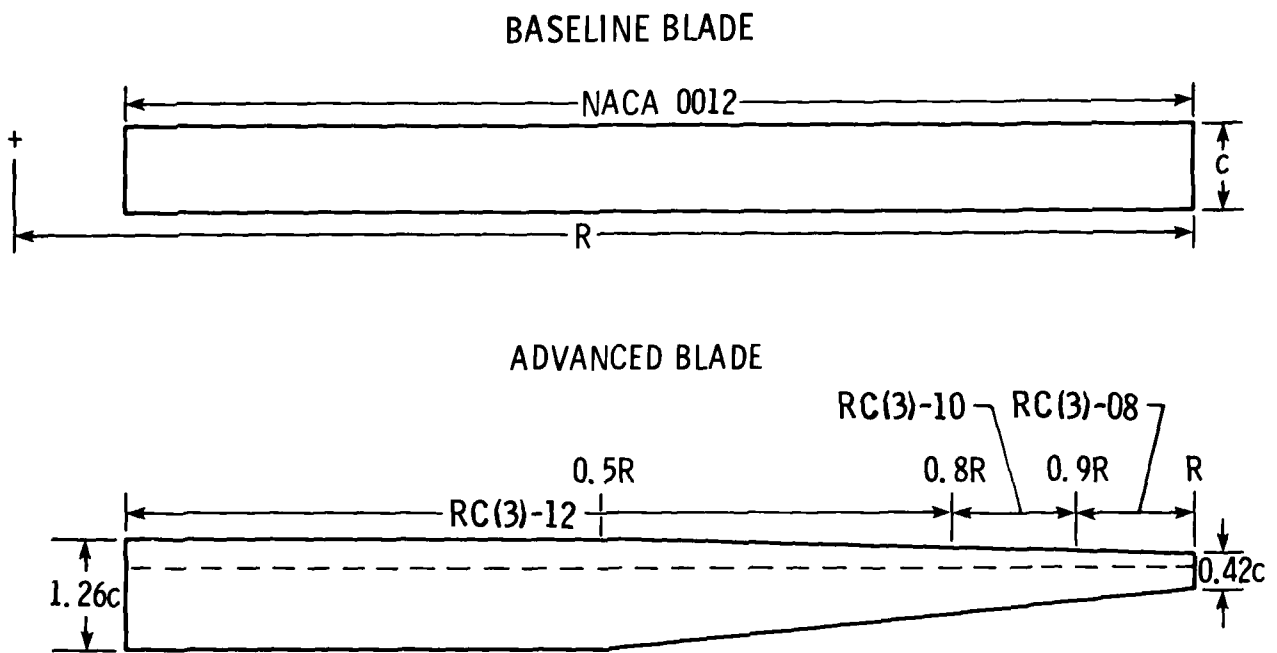
Figure 3.- Blade geometries.
