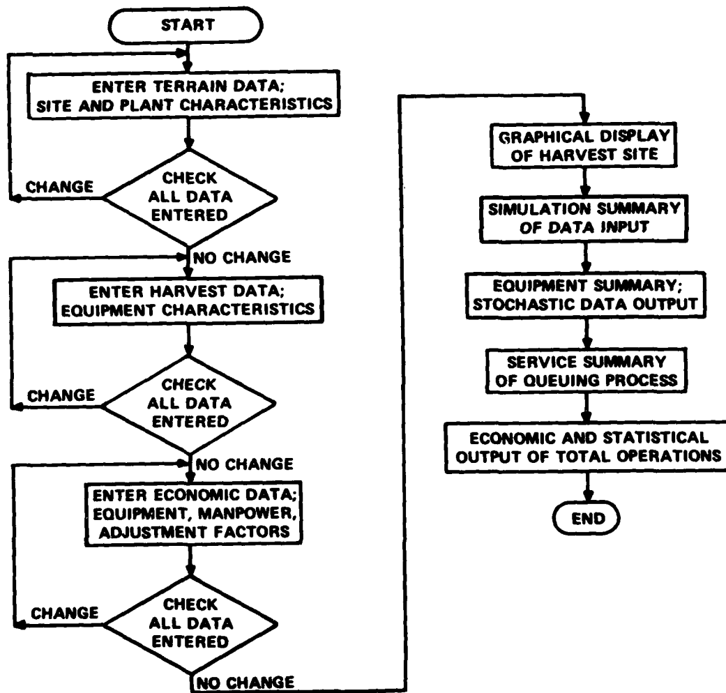
Figure 1. Generalized flowchart for the simulation model SHAP
