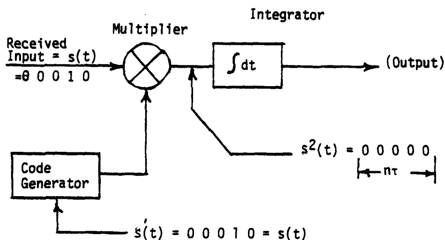
Correlation Detector
