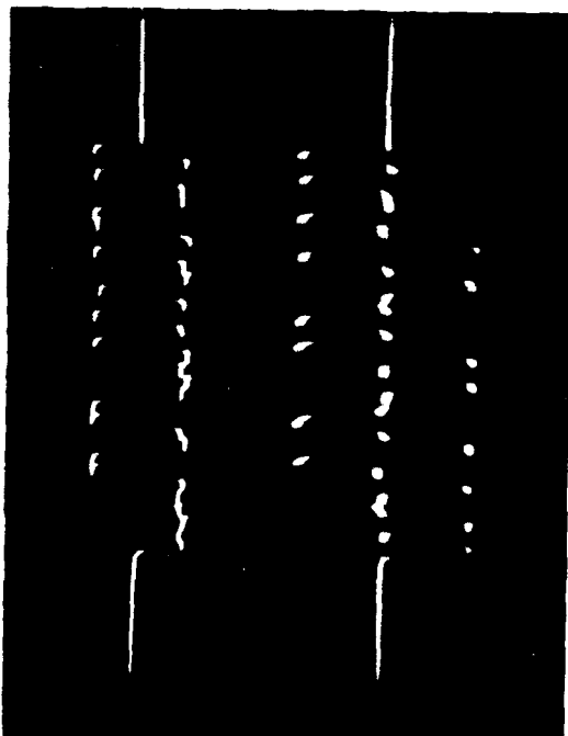
d. INTEGRATOR INPUT (TOP) PHASE DETECTOR OUTPUT OF CODE A (BOT) X + Y SCALES - SAME AS ABOVE
