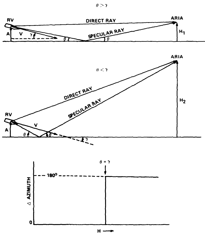
Figure 16. AZIMUTH DIFFERENCE ANGLE DEPENDENCE ON ARIA ALTITUDE FOR AN RV TRAJECTORY IN THE PLANE OF INCIDENCE OF THE SPECULAR RAY
