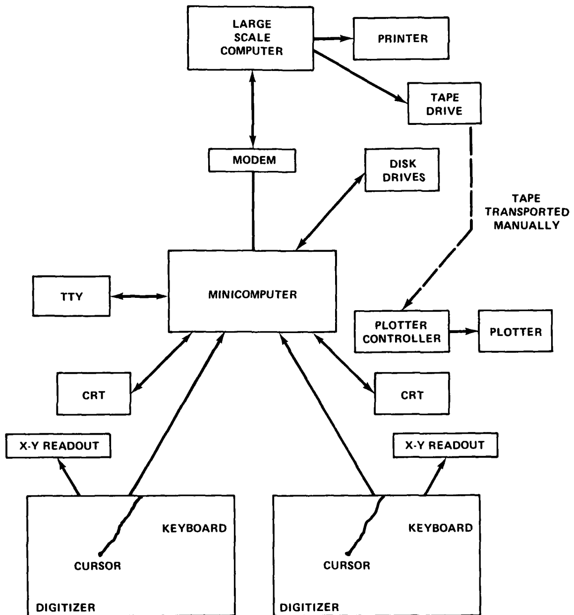
Figure IV-J2 Typical Graphic Data Reduction and Design Station- Two Digitizers
