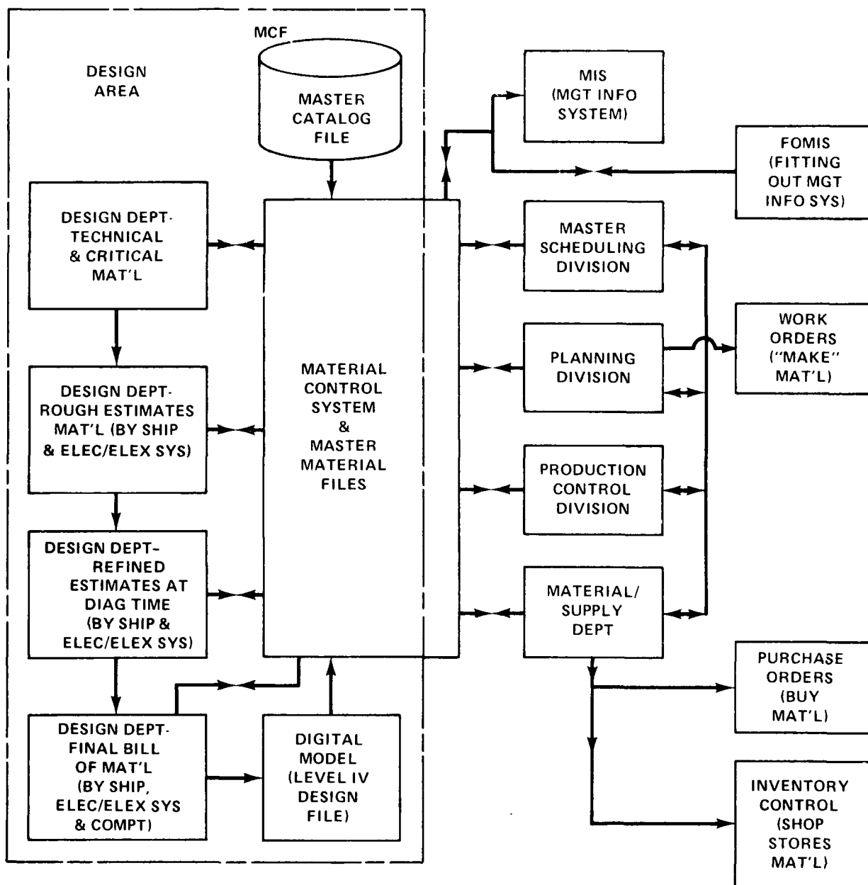
Figure IV-G1 Sheet 2 of 2
