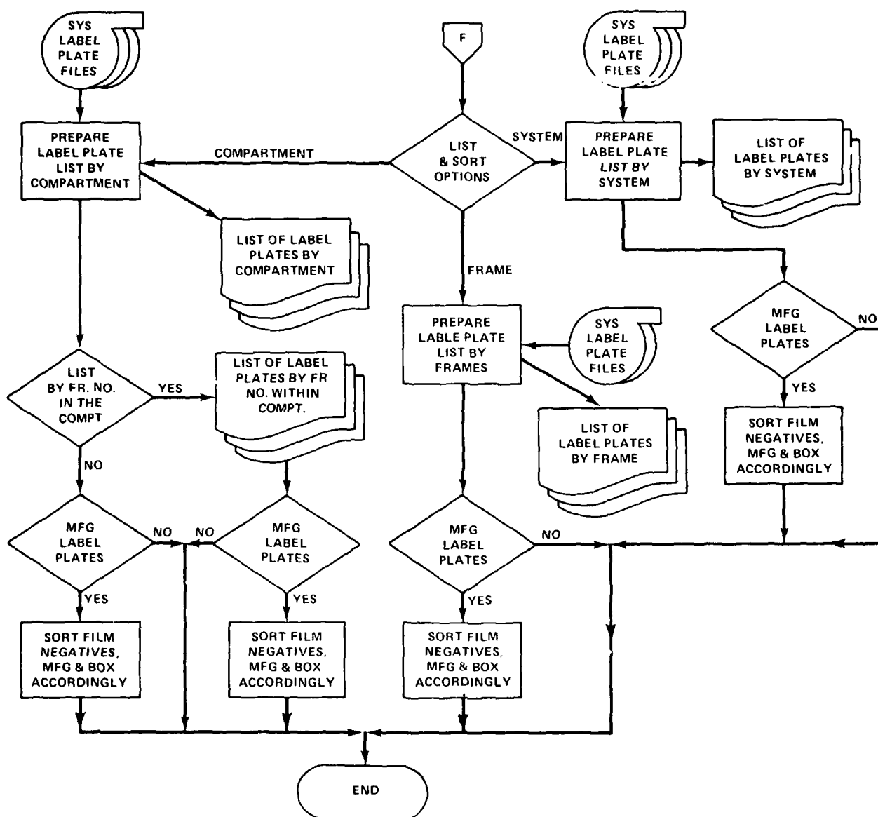
Figure IV-M1 Sheet 5 of 5
