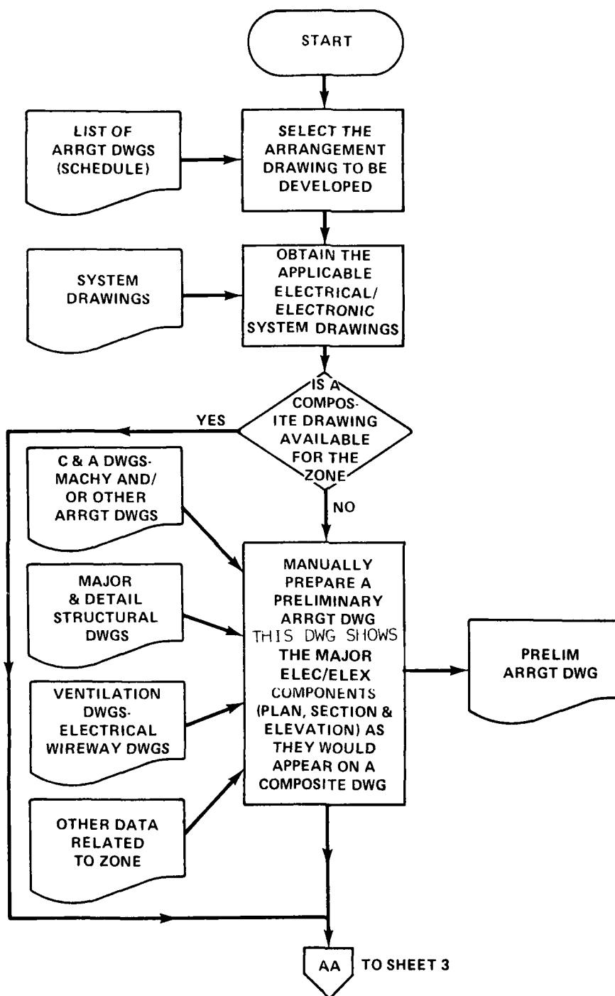
Figure IV-F1 Sheet 2 of 6
