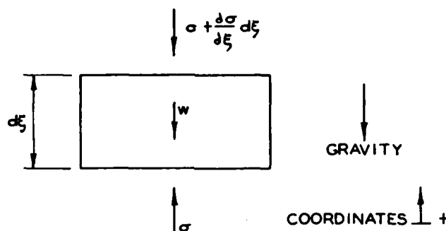
Figure 4. Soil element in equilibrium
