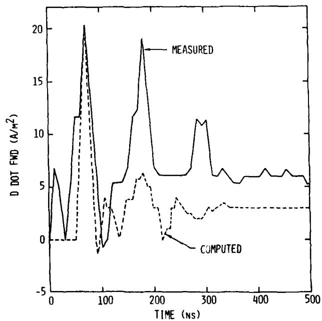
COMPARISON OF MEASURED RESPONSE (FLIGHT 80-18) AND COMPUTED WITH T3DFD AND A 30ns RISE TIME, 590 AMPERE STEP CURRENT SOURCE, NOSE TO TAIL.
