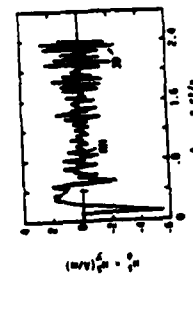
Fig. 16. H_{\theta}^2 = +H_z^2 (unfiltered) at observation point 3 for \epsilon = 2\epsilon_0 .
