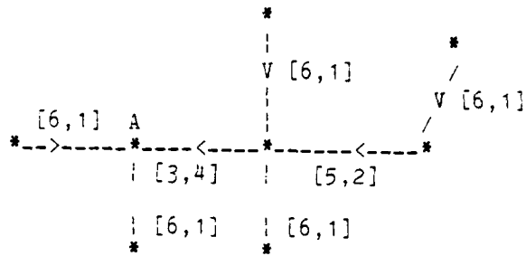
Figure 4.1:2 Example Topology of 7 Clusters Collection at A:Simplex Capacities
