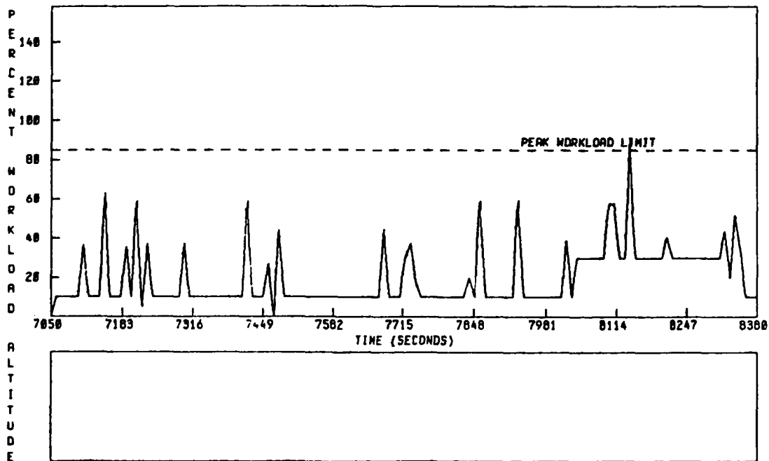
Figure 28 Right Hand Workload Time History
