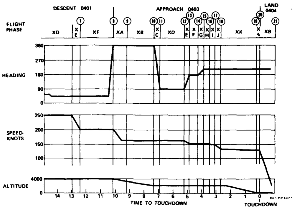
Figure 18 Flight Profile Segment
