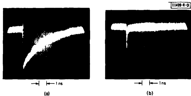
Fig. 1-6. Photoresponse of InP optoelectronic switches to short pulses ( <100 ps) of AlGaAs diode laser ( \lambda \sim 0.85 \mu\text{m} ) with 3-mW peak power. DC voltage of 300 mV was connected between ground and one terminal of device, with response shown observed between other terminal and ground on a high-speed sampling oscilloscope (response time \sim 25 ps). (a) Unbombarded device; (b) device bombarded with a 10^{13} \text{ cm}^{-2} dose of 200-kV protons and subsequently annealed at 250^\circ\text{C} for 10 s.
