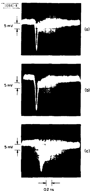
Fig. 1-7. Photoresponse of three InP optoelectronic switches described in Fig. 1-6, following proton bombardment and subsequent 10-s anneal at: (a) 250^\circ\text{C} , (b) 300^\circ\text{C} , and (c) 350^\circ\text{C} .
