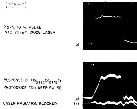
Fig. I-15. Oscilloscope traces of (a) current pulse into a 20- \mu\text{m} \text{PbSnTe} diode laser, (b) response of a \text{Hg}_{0.825}\text{Cd}_{0.175}\text{Te} photodiode to laser pulse, and (c) electrical crosstalk with laser blocked.
