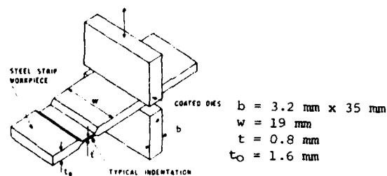
Fig. 2 The plane strain compression test.
