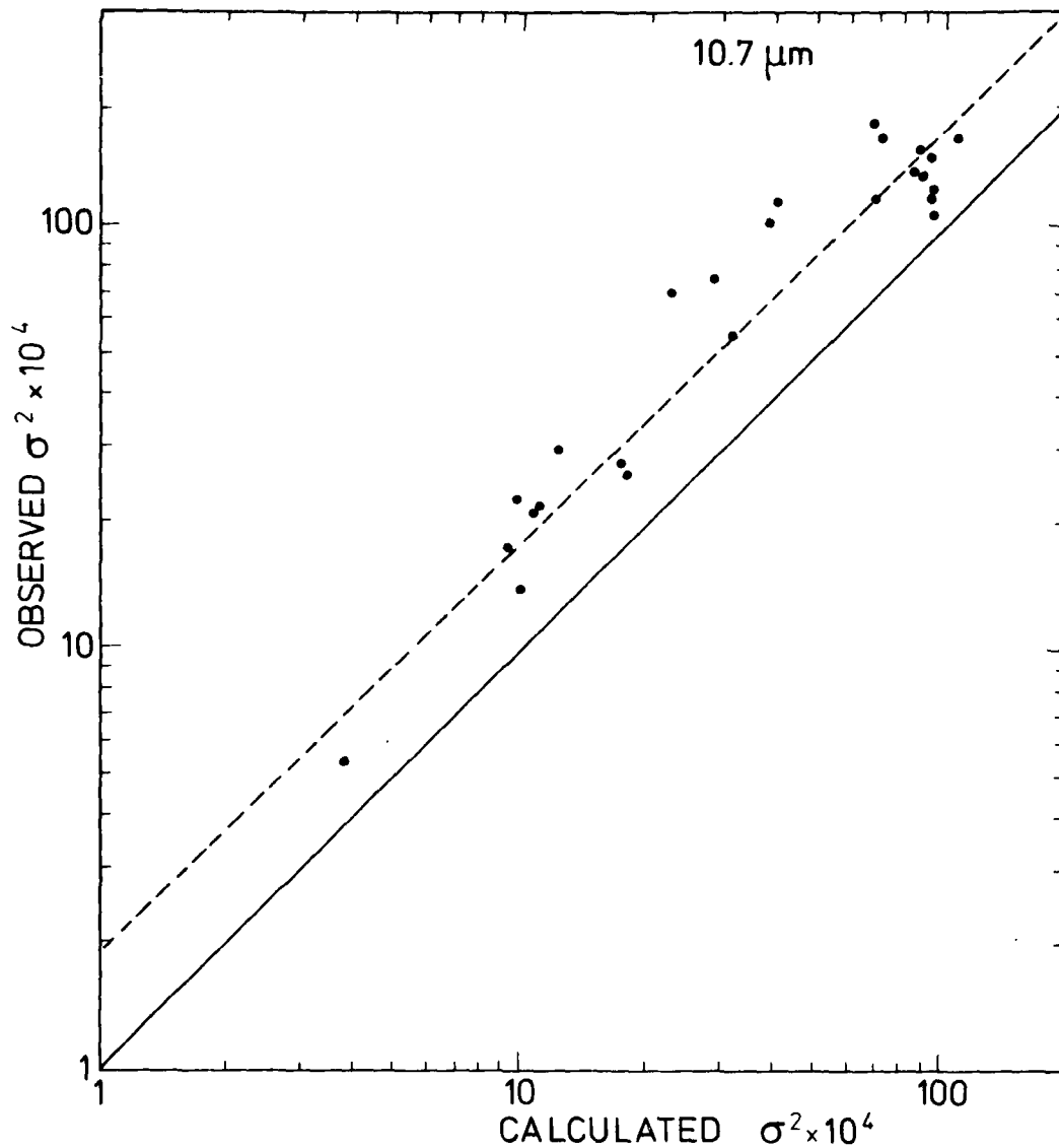
Figure 5.--Observed \sigma^2 [ = \langle (I_A - I_B)^2 \rangle / \langle I \rangle^2 ] of the 10.7- \mu\text{m} \text{CO}_2 scintillometer, compared with the same quantity calculated from measurements of C_T^2 , C_Q^2 , and C_{TQ} .
