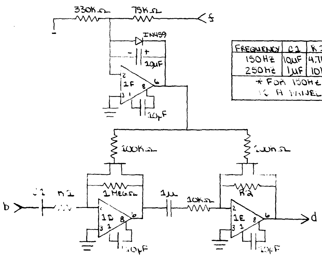
AUTOMATIC GAIN CONTROL CIRCUIT
