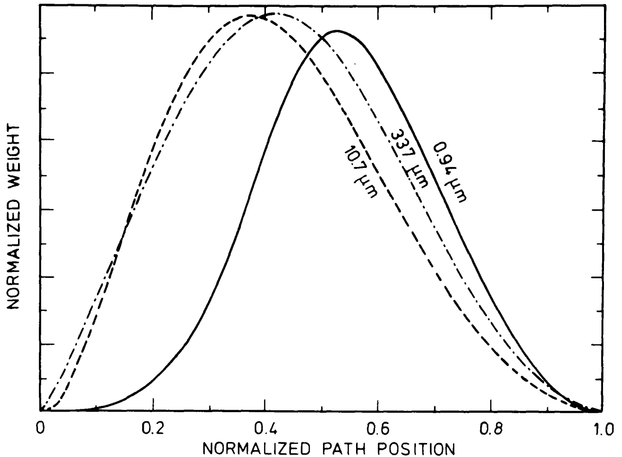
Figure 3.-- C_n^2 path-weighting functions. The 0.94\text{-}\mu\text{m} curve is for a 5-cm tangent aperture receiver, 5-cm transmitter scintillometer. The inner scale is 0.75\text{ cm} for all cases. From R.J. Hill (unpublished).
