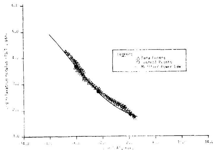
Figure 17. Relationship between \log E(t) and \log t/a_T for Thiokol 177. Legend: Modified Power Law Number 1
