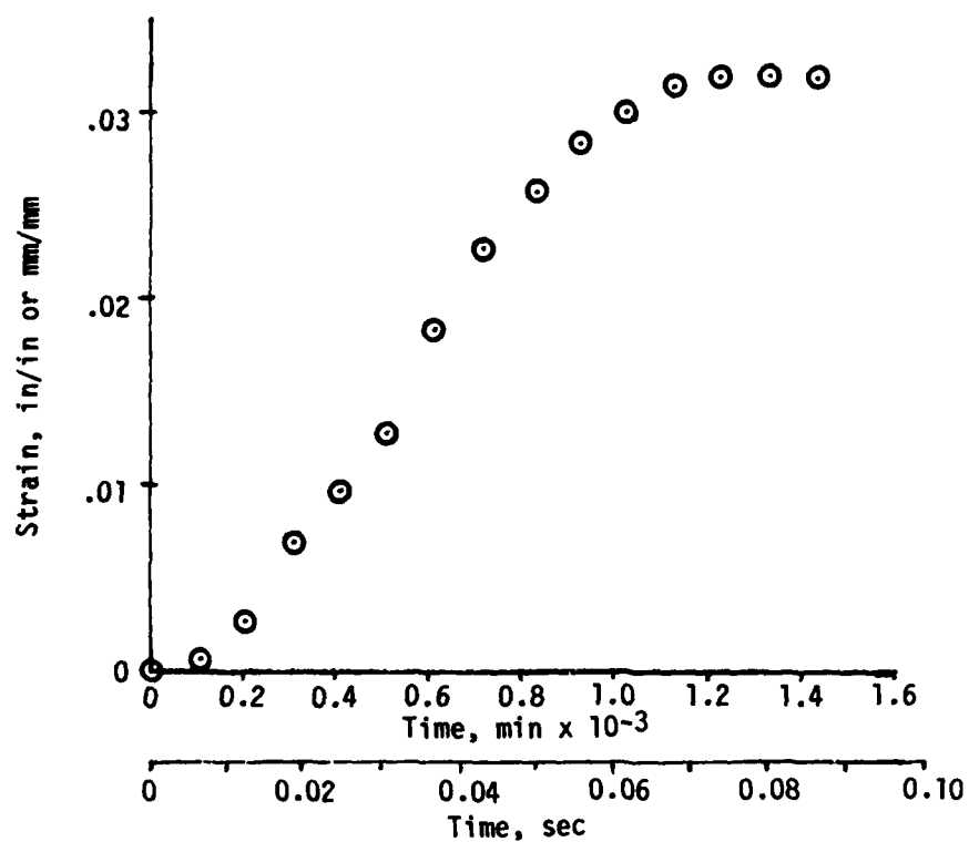
(a) Strain-Time History
