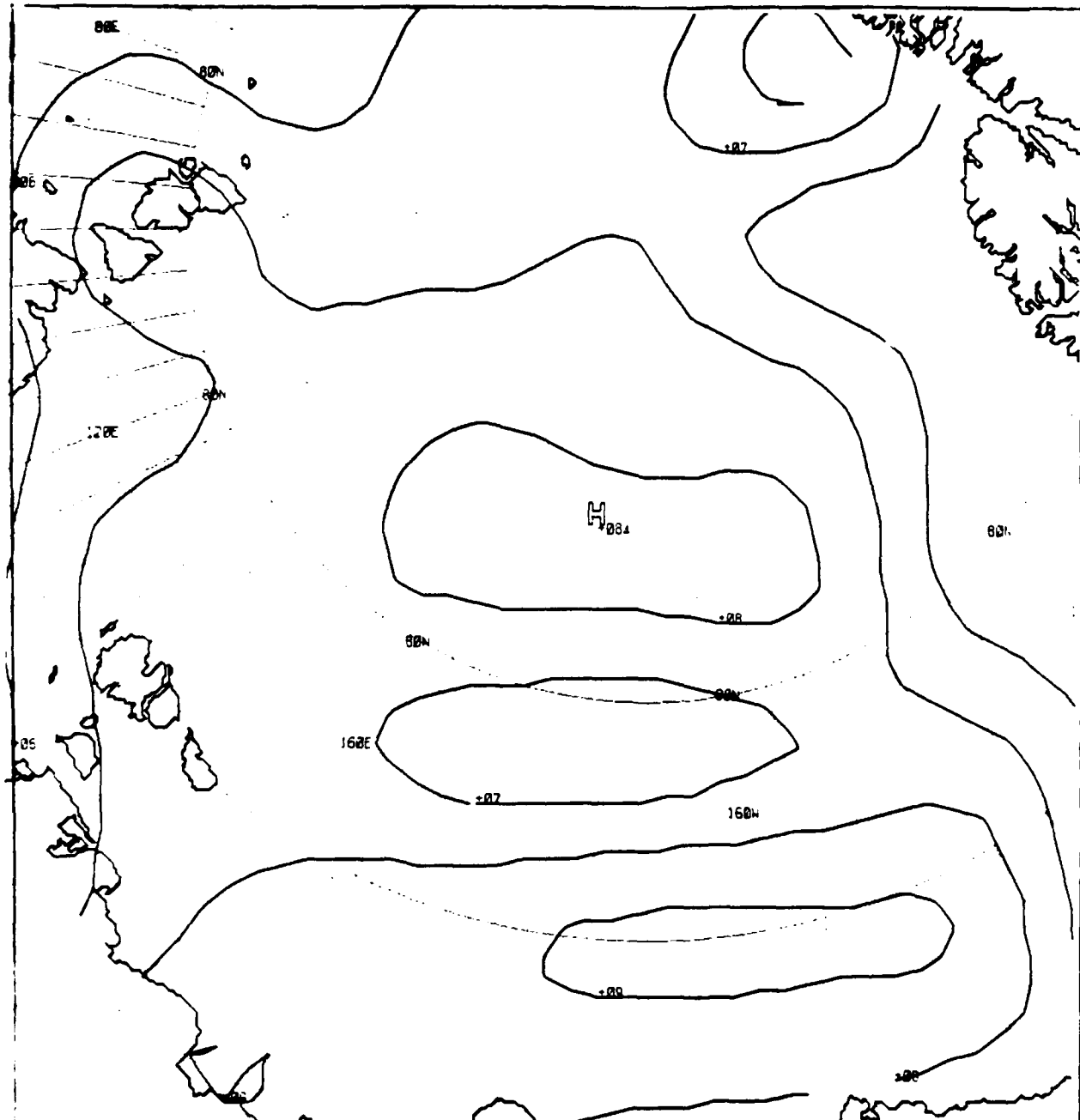
AVERAGE NOVEMBER ICE CONCENTRATION CONTOUR INTERVAL IS 10 PERCENT INCREMENT OF GRID COVERAGE LABELS ARE PERCENT OF GRID CELL COVERED BY THICK ICE DIVIDED
