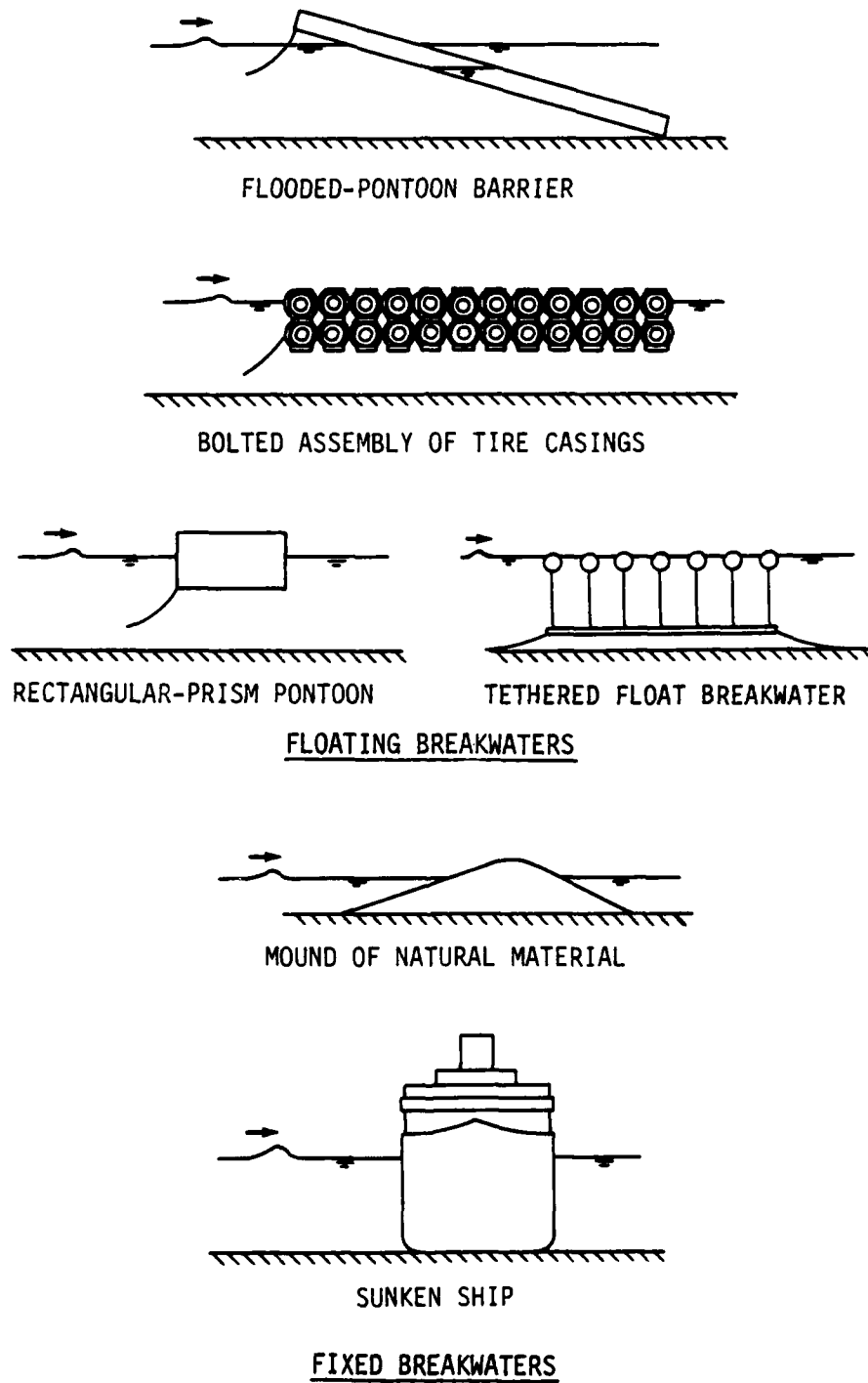
Figure 2.1. Typical Breakwater Configurations
