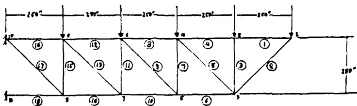
Figure 1. 18-Bar Planar Truss. Initial Geometry.
