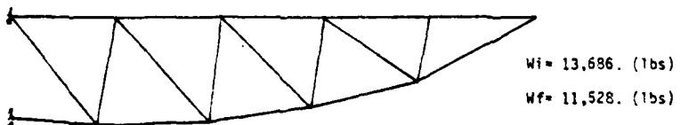
Figure 1d. Stress, Euler Buckling, Displacement, and Frequency.
