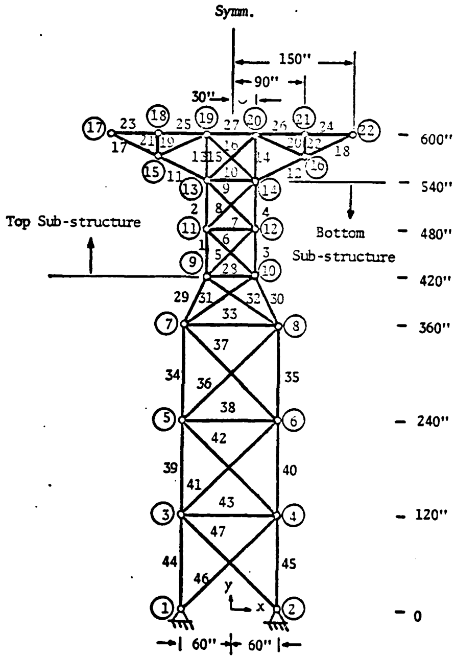
Figure A.6. 47-Bar Planar Tower.
