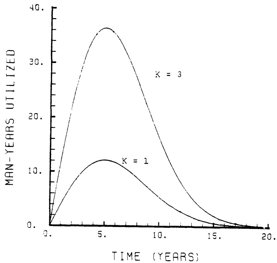
Figure 8 Change in Manpower versus Constant Time-To-Peak [Ref. 13: 159]
