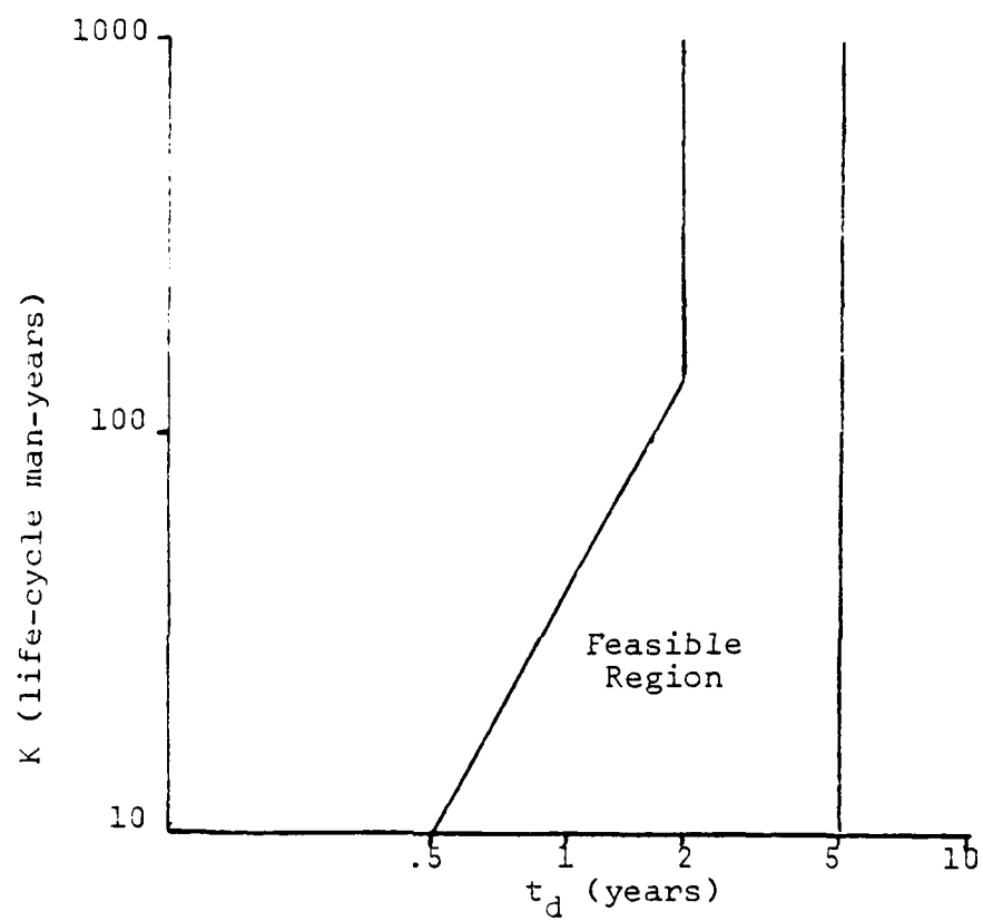
Figure 11 Feasible Software Development Region [Ref. 20: 37]
