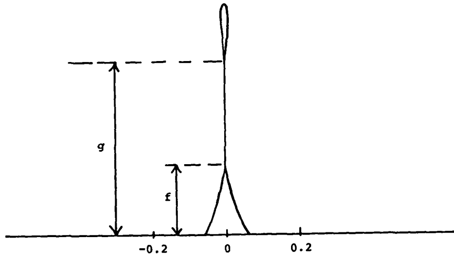
Figure 5. Profile of the bubble with one segment of contact for \gamma = -3.0 and \beta = 2\pi/3 . The vertical scale is the same as the horizontal scale. The values of f and g are respectively 0.19 and 0.47.
