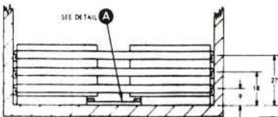
SECTION B-B SHOWING LOCATION OF WALL MEMBERS USED FOR CROSS MEMBERS
