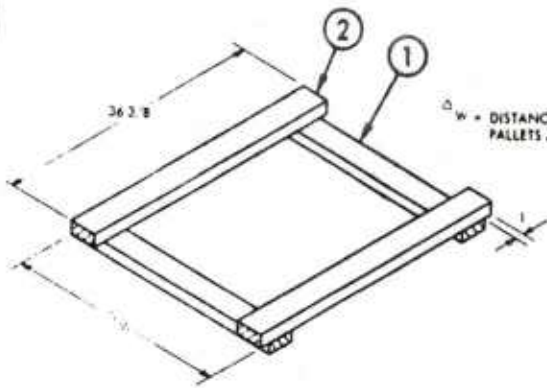
DETAIL A SWAY BRACE FRAME 14 REQUIRED
