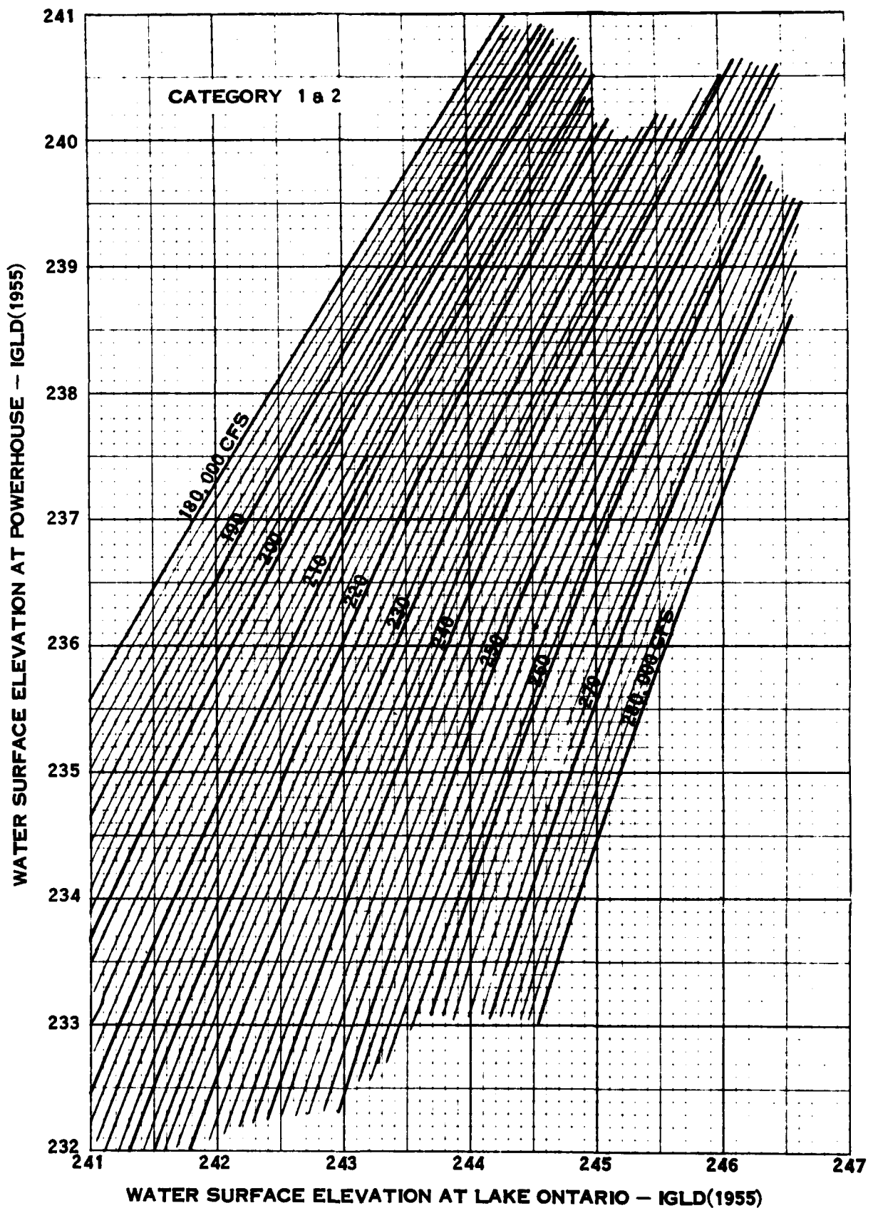
BACKWATER SLOPES LAKE ONTARIO TO MOSES-SAUNDERS POWERHOUSE ICE COVER CONDITION
