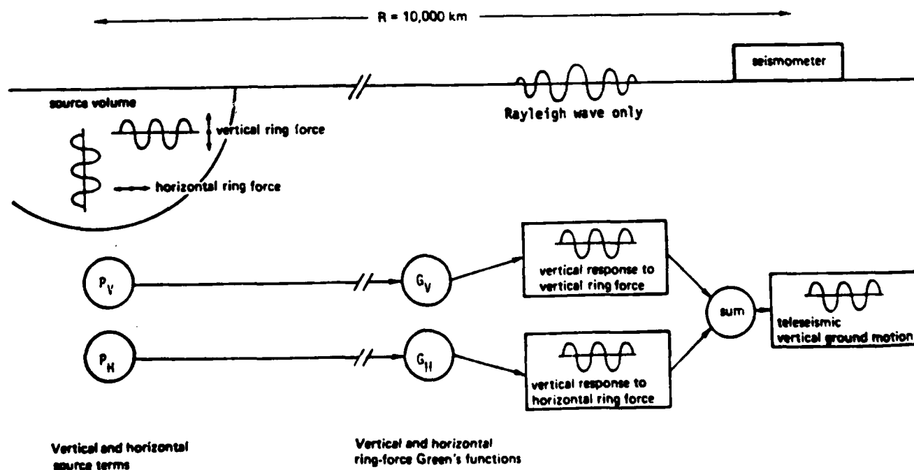
Fig. 2--Schematic outline of PSR M_v model showing source terms, propagators, and vertical response for one harmonic component and one ring force. Complete vertical response requires a summation over all rings and all harmonic components.
